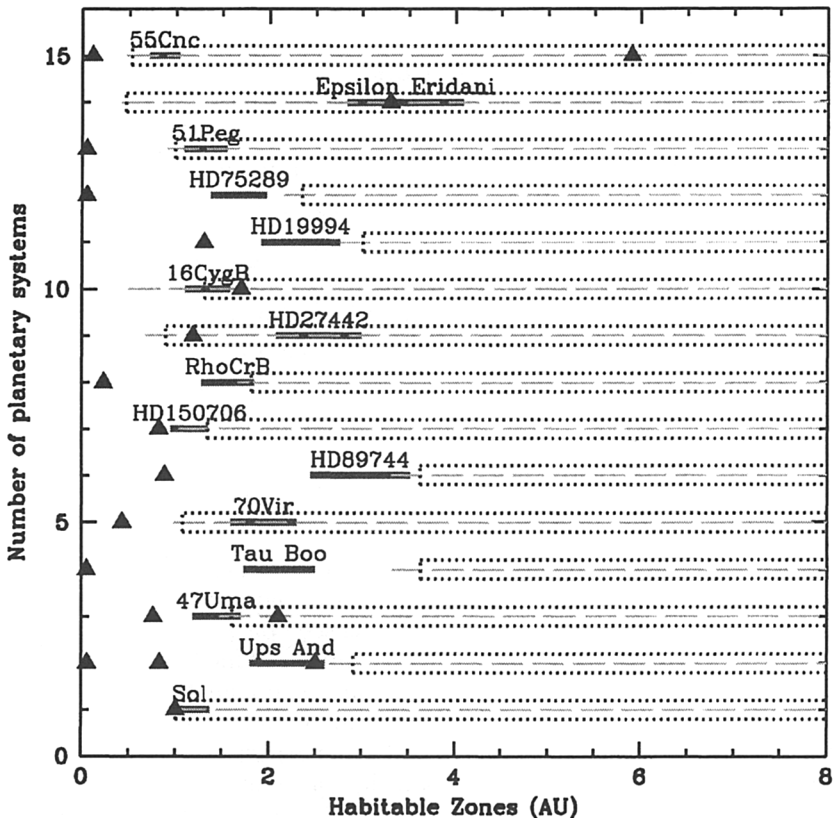
Figure 1. Habitable zones for visible and UV radiation
