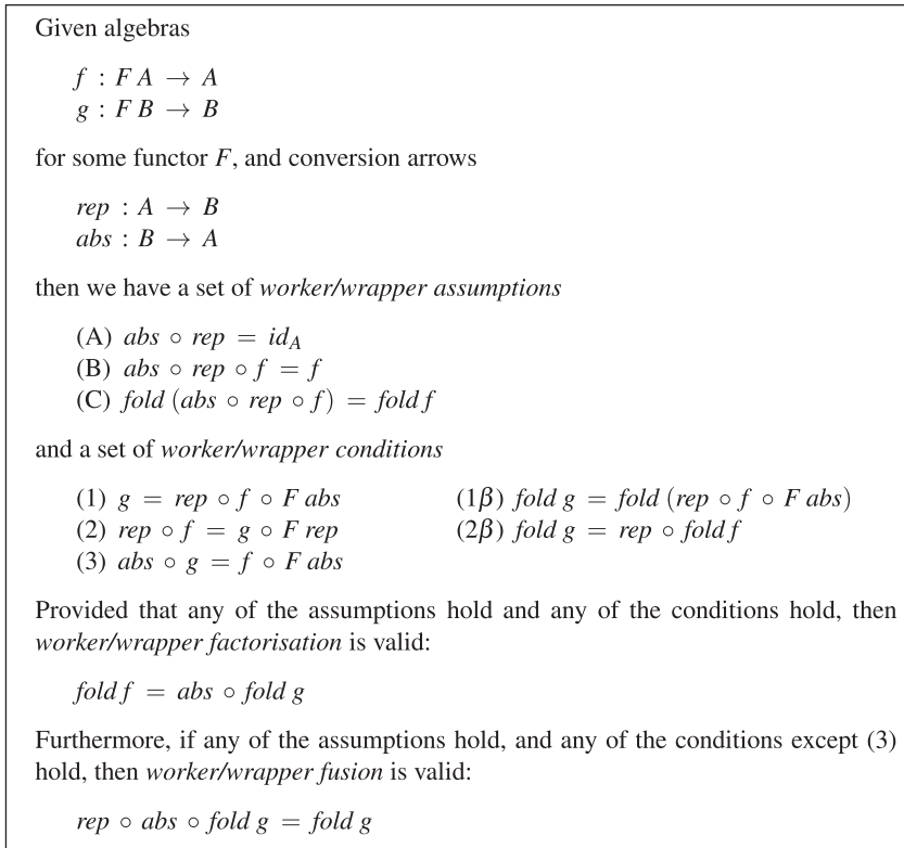
Fig. 2. Worker/wrapper transformation for initial algebras.
