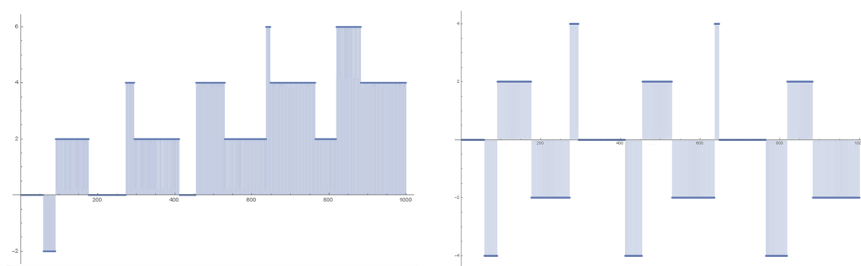
Figure 3: \sigma_K(\omega) for K = T_{2,17} \# -2T_{2,11} and K = 2T_{2,17} \# -3T_{2,11} .
