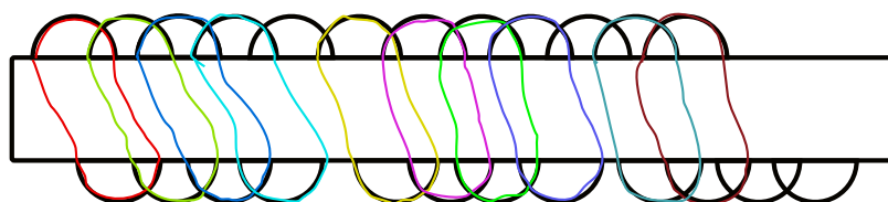
Figure 2: A schematic of a Seifert surface for T_{2,13} - 3T_{2,5} and surgery curves.
