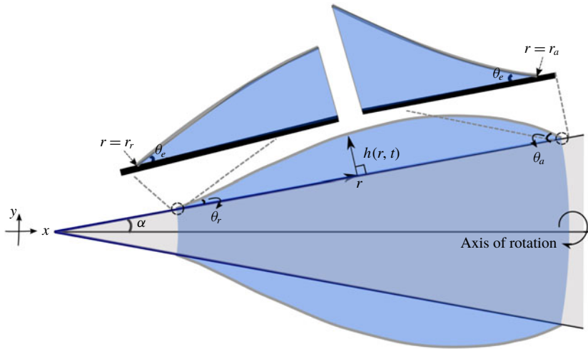
FIGURE 1. Sketch of a droplet on a conical fibre with an angle \alpha . The droplet shape is described by the height h(r, t) from the substrate to the free surface as a function of the radial distance from the vertex along the substrate r and time t . At the contact line positions, i.e. r = r_r and r = r_a , the free surface intersects with the substrate with an equilibrium (microscopic) contact angle \theta_e . The free surface deforms significantly in the vicinity of the contact line due to a large viscous stress. At the droplet scale, the contact angle appears as the apparent contact angles, \theta_r at the thinner part of the cone (receding contact line) and \theta_a at thicker part of the cone (advancing contact line).
