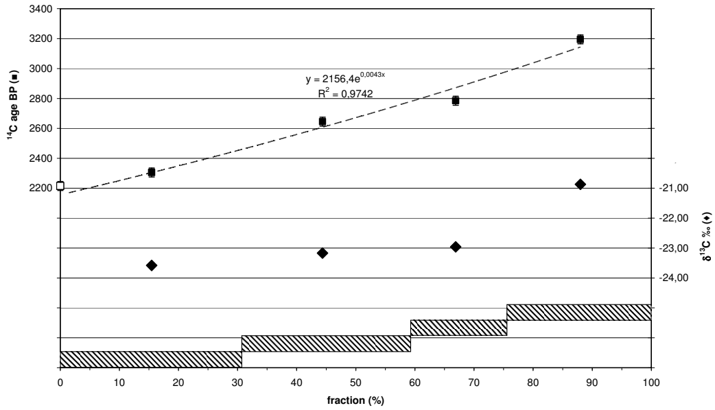
Figure 5 The 4 dated lime fractions (filled squares) and a charcoal (empty square) inclusion from Sant Joan de Misa
