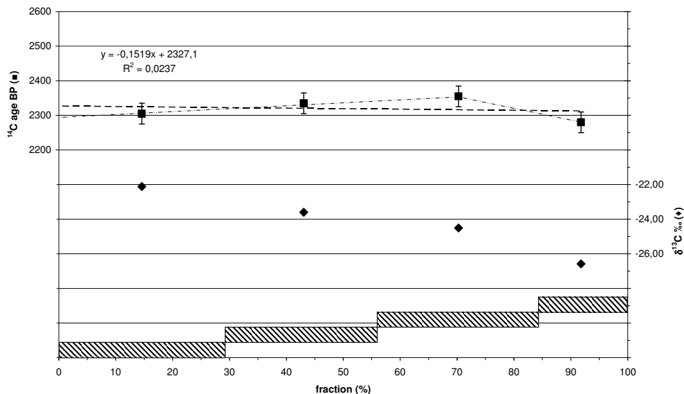
Figure 10 The 4 dated lime fractions from Muertos Gallard (skull and hair band)
