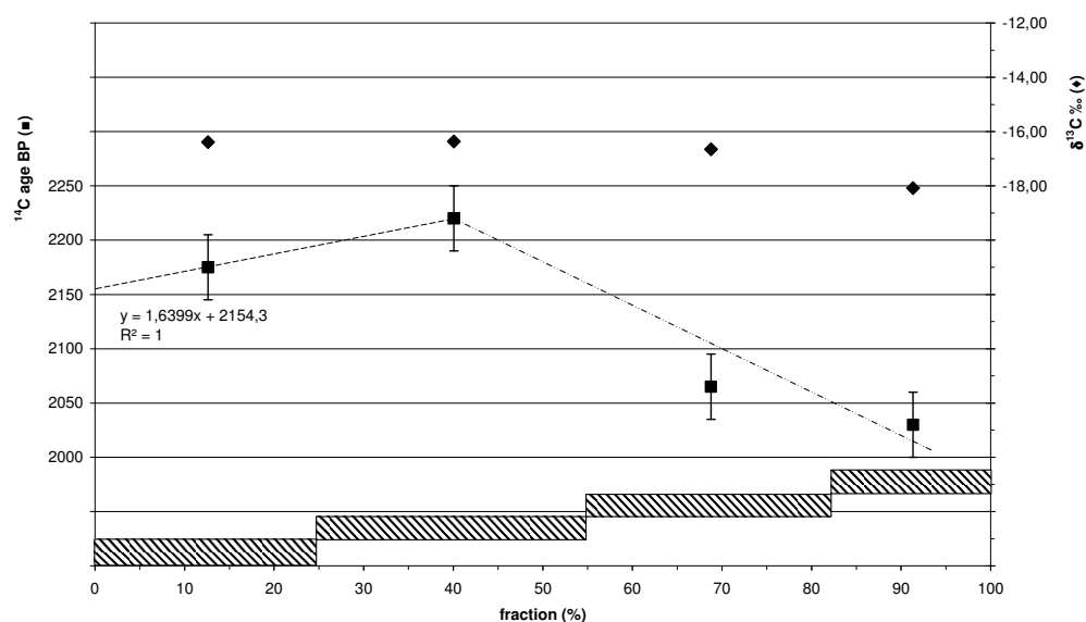
Figure 7 The 4 dated lime fractions from Muertos Gallard (lime pit)
