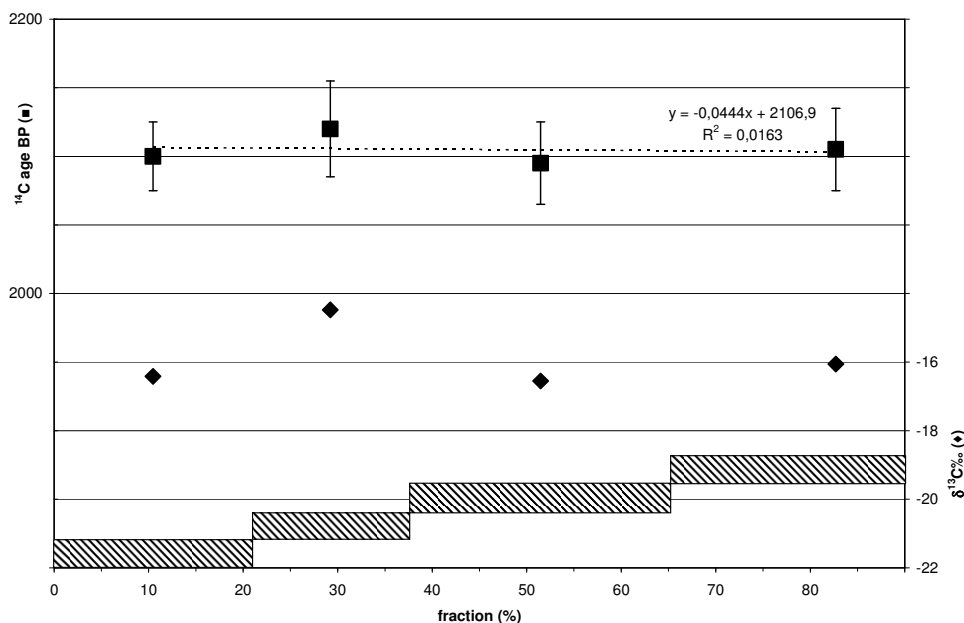
Figure 4 The 4 dated fractions from Binigaus
