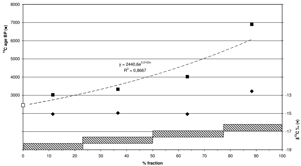
Figure 6 The 4 dated lime fractions (filled squares) and charred grain (empty square) from Son Oms
