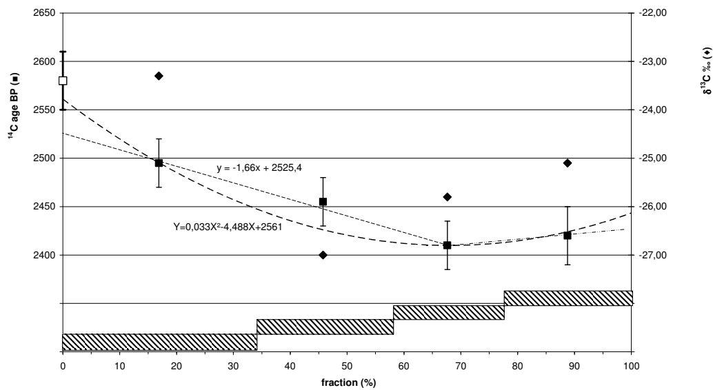
Figure 9 The 4 dated lime fractions (filled squares) from Son Matge (ref. 2200–2204) and 1 carbon black sample from a burnt bone (empty square).
