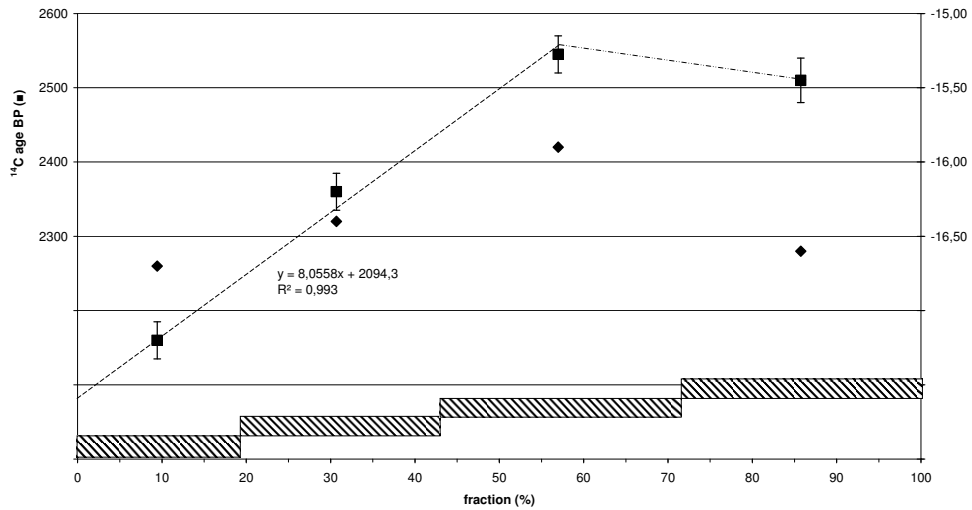
Figure 8 The 4 dated lime fractions from Son Matge (outside Talayotic wall)
