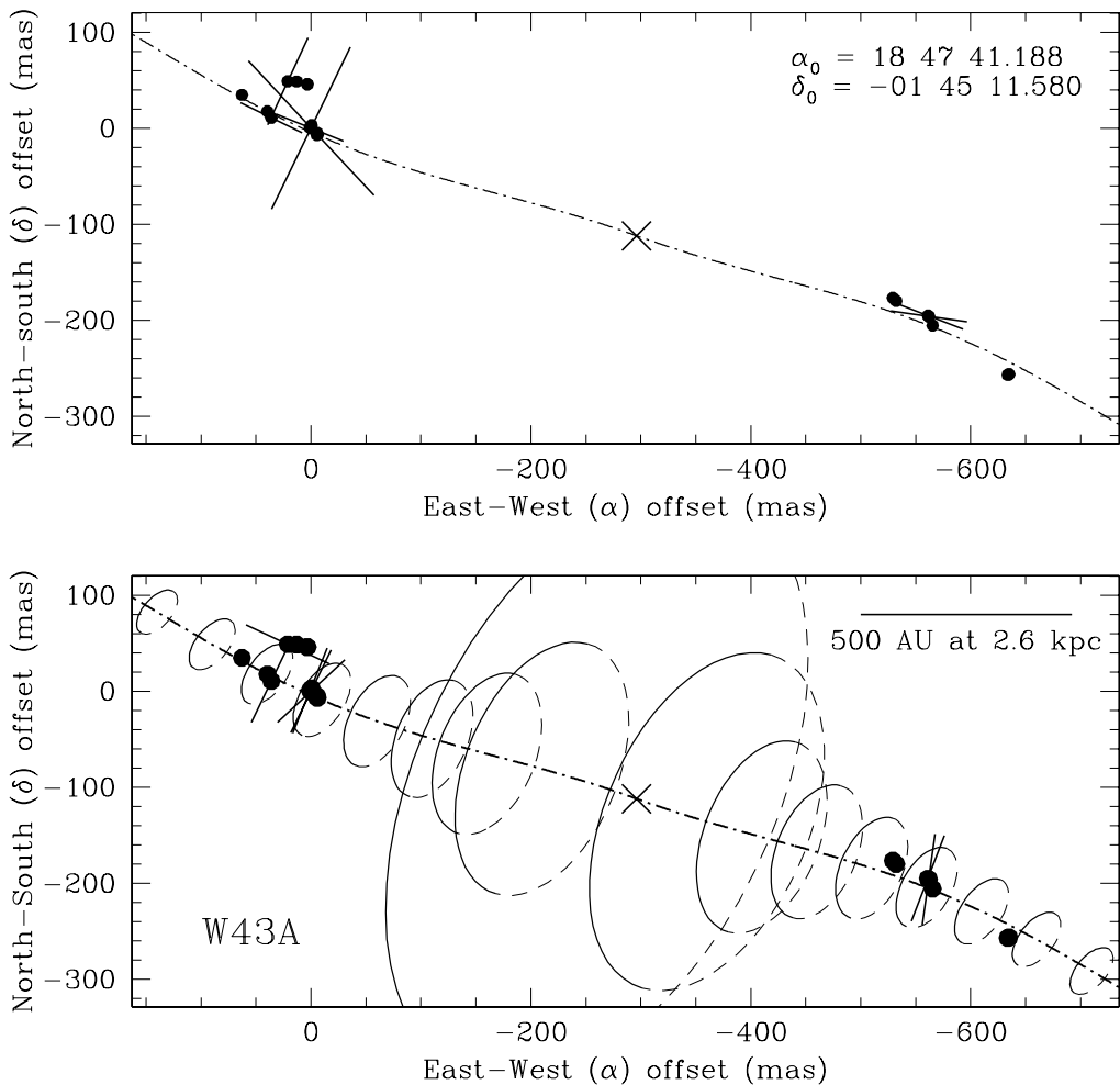
Figure 1. The \text{H}_2\text{O} masers in the precessing jet (dashed-dotted line) of W43A (indicated by the cross). (top): The maser features with the determined linear polarization vectors scaled linearly according to the fractional linear polarization. The polarization vectors lie predominantly along the jet with a median angle of \chi = 63 \pm 12^\circ east of north. (bottom): The toroidal magnetic field of W43A. The vectors indicate the determined magnetic field direction, perpendicular to the polarization vectors, at the location of the \text{H}_2\text{O} masers. The ellipses indicate the toroidal field along the jet, scaled with magnetic field strength \propto r^{-1} .
