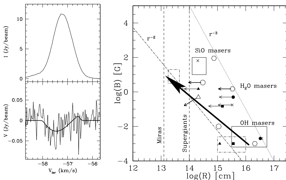
Figure 2. (left): The total intensity and circular polarization spectrum of the H 2 O maser feature for which circular polarization was detected. (right): The figure, reproduced from Vlemmings et al. (2005), of measured magnetic fields for the masers in the CSEs of evolved stars. The dashed-dotted boxes indicate the range of magnetic field strengths measured for the SiO and OH masers of Mira stars and the solid boxes those of supergiant stars. The thin arrows indicate the H 2 O maser magnetic fields measured by Vlemmings et al. (2002) and Vlemmings et al. (2005), where the lengths of the arrows indicate the thickness of the H 2 O maser shell with the symbols drawn on the outer edge. The symbols without arrows are the measurements on SiO and OH masers from the literature on the same sample of stars. The thick solid arrow indicates the magnetic field in the jet of W43A.
