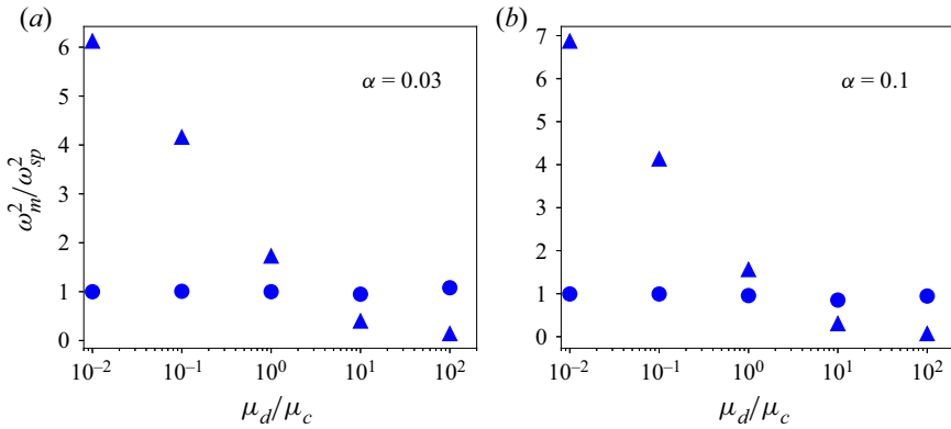
Figure 12. Phase-averaged entropy \omega_m^2 (normalized by its value in the single-phase case SP1) for different viscosity ratios \mu_d / \mu_c . Triangles indicate the dispersed phase ( m = d ), while circles indicate the carrier phase ( m = c ). (a) Results for \alpha = 0.03 ; (b) results for \alpha = 0.1 .
