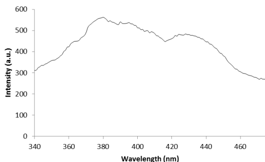
Figure 2a Excitation spectrum between 340 and 475 nm of uncontaminated wool fibers. Excitation band centers are observed at 380 and 430 nm.
