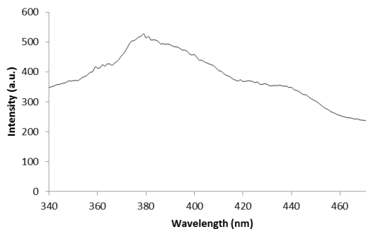
Figure 2b Excitation spectrum between 340 and 475 nm of uncontaminated silk fabric. The excitation band center is observed at 378 nm.
