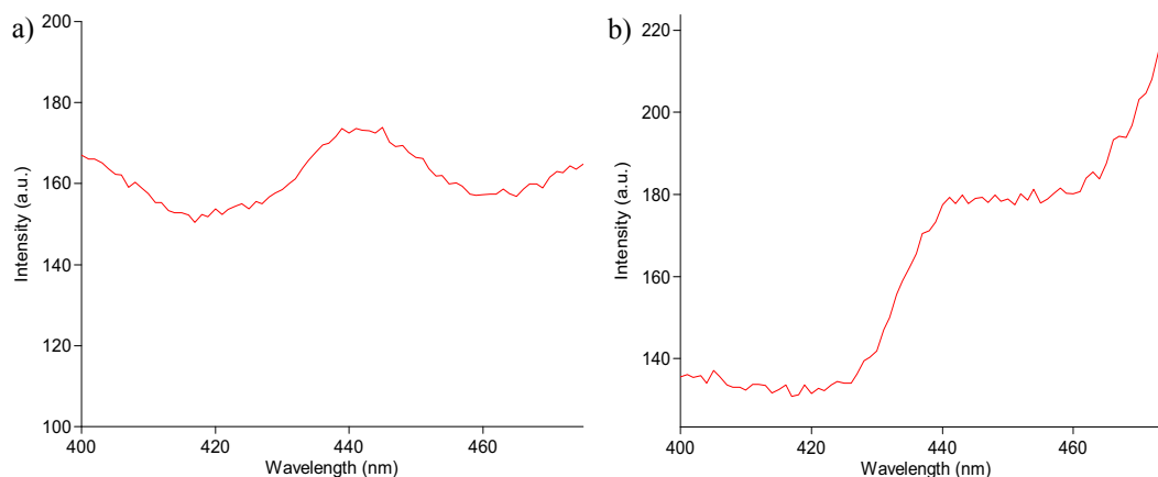
Figure 4 Excitation spectra of modern silk fabric immersed in mixture of humic substance (Roth) and Milli-Q water during 64 hr (a) and 188 hr (b).
