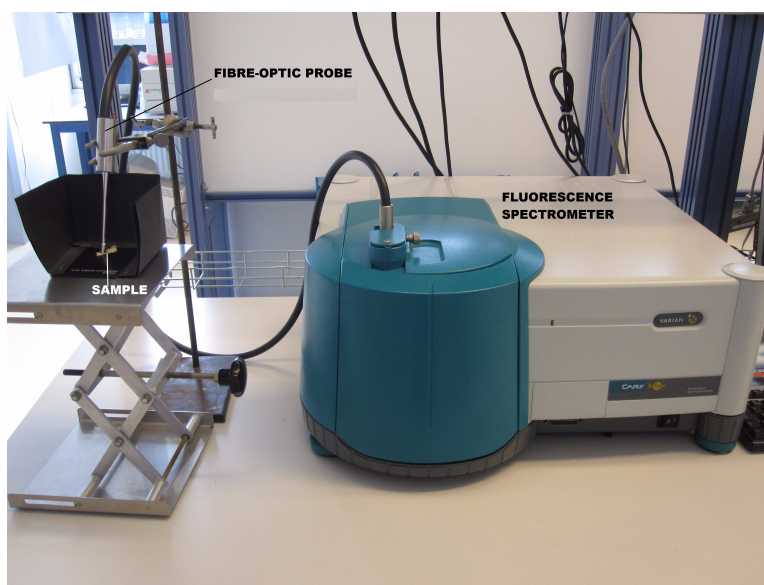
Figure 1 Varian Cary Eclipse fluorescence spectrophotometer with a fiberoptic probe
