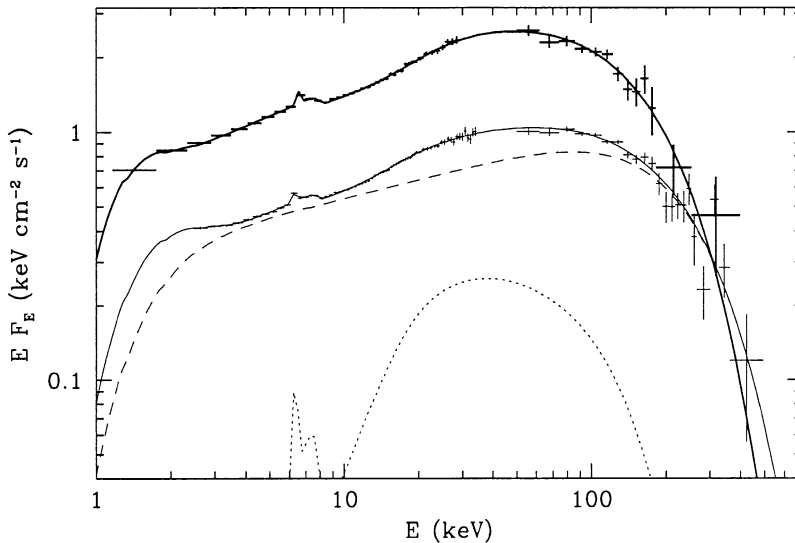
Figure 2. X \gamma spectra of GX 339–4 in the hard state from simultaneous observations by Ginga -OSSE (upper spectrum: Z98) and RXTE-OSSE (lower spectrum: Zdziarski et al., in preparation). The spectra are fitted by the sum of blackbody, thermal Comptonization, and Compton reflection including an Fe K \alpha line. The last two components are shown for the lower spectrum by the dashed and dotted curves, respectively.
