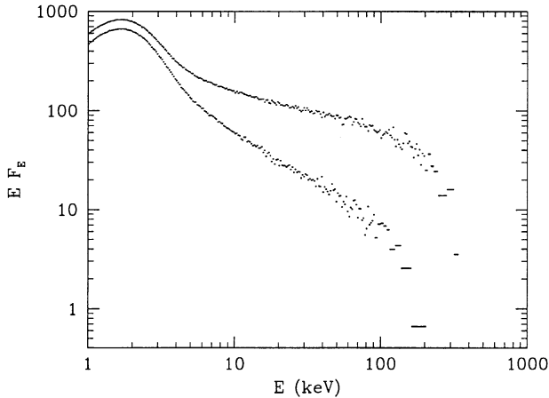
Figure 5. Spectra in the BMC model simulated by LT99 (statistical errors are comparable to the scatter of the points). The lower and upper spectra correspond to \dot{m} = 2 and 4, respectively. The free-falling electrons were assumed to have kT = 5 and 20 keV, and the power-law parts of the spectra have \Gamma \simeq 2.9 and 2.5, respectively.
