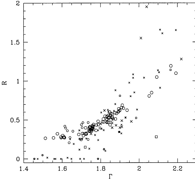
Figure 8. Values of \Gamma and R in the hard state of BH binaries (open circles; same as in Figure 3) and neutron-star binaries (open squares), in Seyfert 1s (crosses) and broad-line radio galaxies (asterisks). Large and small symbols correspond to RXTE and Ginga data, respectively. For clarity, error bars are not shown.
