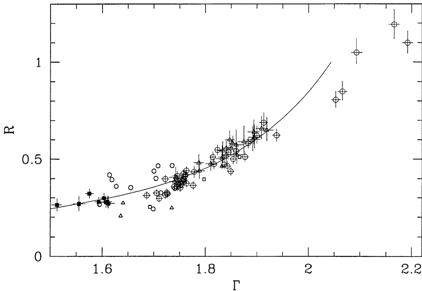
Figure 3. Correlation between the strength of Compton reflection and the X-ray spectral index in BH binaries. Larger symbols with error bars and smaller ones without them correspond to observations by RXTE and Ginga , respectively. Open circles, triangles, squares, and filled squares correspond to Cyg X-1, GX 339-4, Nova Muscae, and GS 1354-644, respectively. The solid curve corresponds to the model of ZLS99 in the geometry shown in Figure 4.
