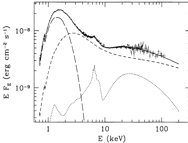
Figure 7. The soft-state spectrum of Cyg X-1 from an ASCA-RXTE observation fitted by Comptonization by nonthermal electrons (dominating above the break seen in the short-dashed curve at \sim 15 keV) as well as by thermal ones (the short-dashed curve below the break), of disk blackbody photons (long dashes), and Compton reflection from the disk (dots).
