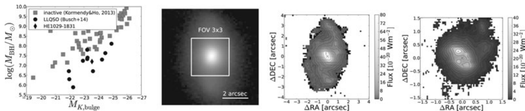
Figure 1. From left to right: (1) In the M_{\text{BH}} - L_{\text{bulge}} relation, the observed LLQSOs clearly lie off set compared to inactive galaxies collected by Kormendy & Ho (2013) (see Busch et al. 2014). (2) K -band image of the LLQSO HE 1029-1831 from Fischer et al. (2006). (3) Pa \alpha map of HE 1029-1831 with a FOV of 8 \times 8 arcsec 2 . (4) the same with FOV of 3 \times 3 arcsec 2 . The atomic gas is distributed in spiral arms and a clumpy circum-nuclear ring, indicating star formation. This motivates further investigation of the star formation properties in the centers of LLQSOs.
