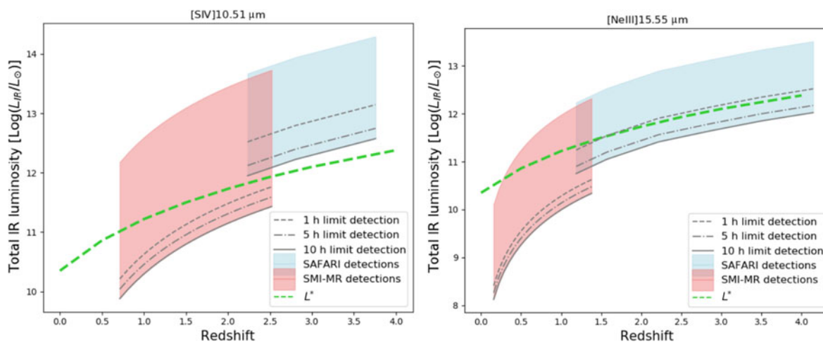
Figure 13. Redshift-luminosity diagrams simulating low-metallicity galaxies detections with SAFARI and SMI-MR mode. (a: left:) Detectability of the [S IV]10.51 \mu\text{m} line. The same colour code is applied as in Figure 10. (b: right:) Detectability of the [Ne III]15.6 \mu\text{m} line.
