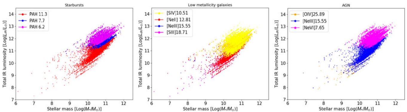
Figure 4. Stellar mass-luminosity diagrams of galaxies detectable in the SMI 1 deg 2 ultra-deep survey from the HELP database. (a: left) Star-forming galaxies. (b: center) Low-metallicity galaxies. (c: right) AGN.
