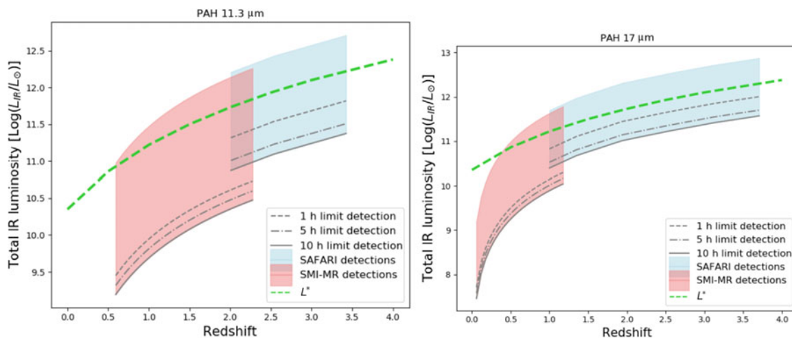
Figure 12. Redshift-luminosity diagrams simulating the SF galaxies detections with SAFARI and SMI-MR mode. (a: left:) Detectability of the PAH 11.3 \mu\text{m} band. The same colour code is applied as in Figure 10. (b: right:) Detectability of the PAH 17.0 \mu\text{m} band.
