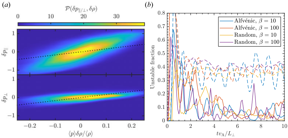
FIGURE 2. (a) Probability distributions of fluctuations in p_{\parallel} , p_{\perp} and \rho , for \beta = 10 Alfvénically driven turbulence. The black dotted lines represent a slope of 5/3, the expectation for single-adiabatic, collisional MHD. Neither \delta p_{\parallel} nor \delta p_{\perp} appear to align with the MHD prediction or with each other. (b) The fraction of the domain whose pressure anisotropy lies beyond the microinstability thresholds as a function of time for all active- \Delta (solid) and passive- \Delta (dashed) simulations. The passive- \Delta simulations typically have \sim 50\% of their volume unstable, whereas the unstable fraction of the active- \Delta simulations typically remains below 10%.
