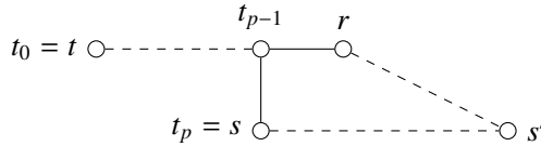
FIGURE 1. Illustration for the proof of Lemma 4.4.
