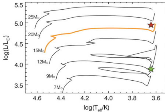
Figure 3. Plot showing the effect of including the additional reddening we observe on progenitor mass estimates for star #1. The green star represents the mass estimate when no circumstellar extinction is considered, the red star shows the estimated progenitor mass when we take into account additional extinction and the orange line shows the best fit mass track for this cluster. The mass tracks are from Georgy et al. (2013) and are at Z = 0.002 .
