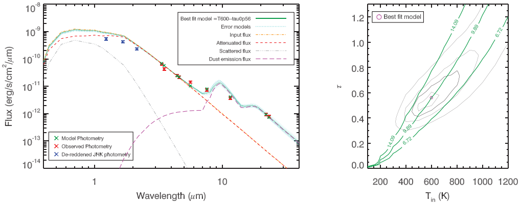
Figure 1. Left panel: Model plot for the star with the highest \dot{M} value in NGC 2100 including all contributions to spectrum. Right panel: Contour plot showing the degeneracy between \chi^2 values and best fitting \dot{M} values in units of 10^{-6} M_{\odot} \text{ yr}^{-1} . The green lines show the best fit \dot{M} and upper and lower \dot{M} isocontours. It can be seen that while there is some degeneracy between inner dust temperature and optical depth the value of \dot{M} is independent of this. Figures taken from Beasor & Davies (2016).
