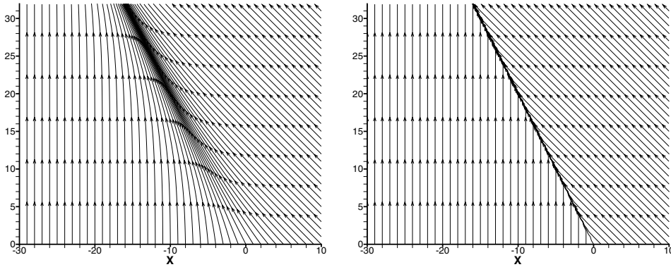
Figure 2.2. The curves \{(x(t), t) : \dot{x} = f'(\varphi(\frac{x-ct}{\epsilon}))\} for \epsilon = 1 (left) and \epsilon = 0.1 (right) for the case \phi^- = 1/2 and \phi^+ = 1 .
