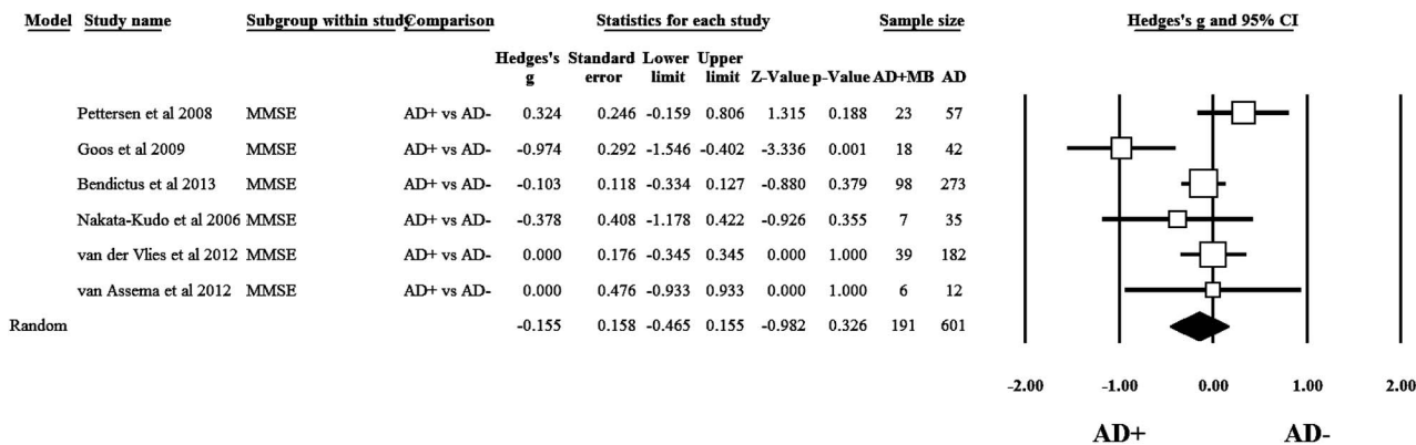
Figure 1: Forest plot showing standardized mean difference on MMSE scores for AD + MB and AD-MB.
