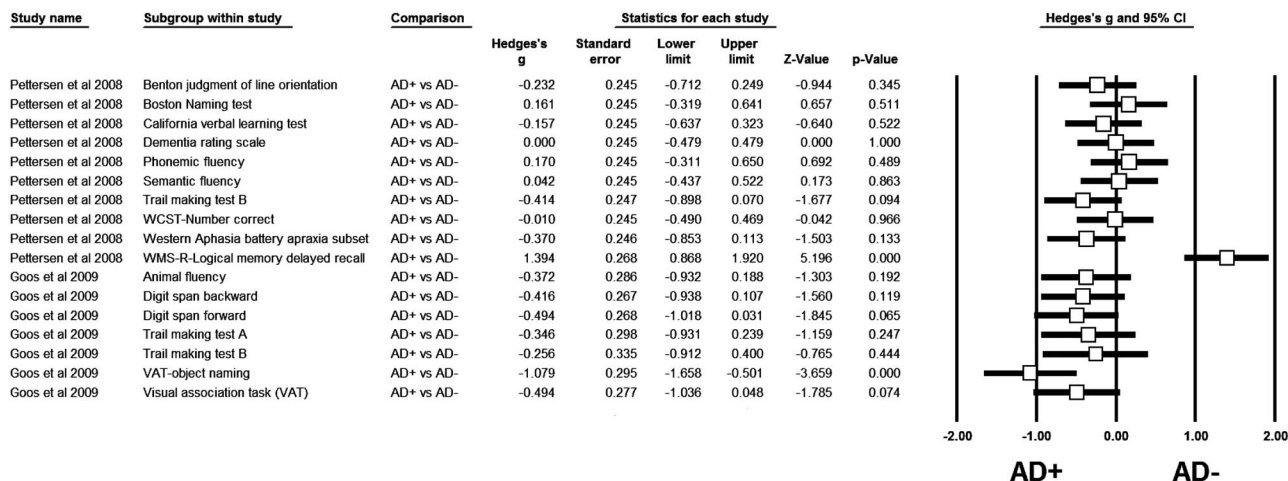
Figure 2: Presentation of the standard difference in means per scales and studies.
