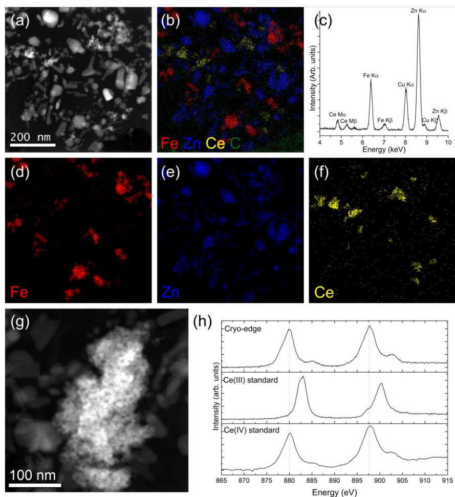
Figure 1. Cryo-analytical STEM of a model nanoparticle mixture. (a) Cryo-HAADF-STEM image with corresponding EDX maps and spectrum (b – f). (g) Cryo-HAADF STEM image with (h) EELS spectrum from the area compared to standard spectra (non-cryo) confirming the agglomerated CeO 2 nanoparticles in suspension retain a Ce(IV) oxidation state.
