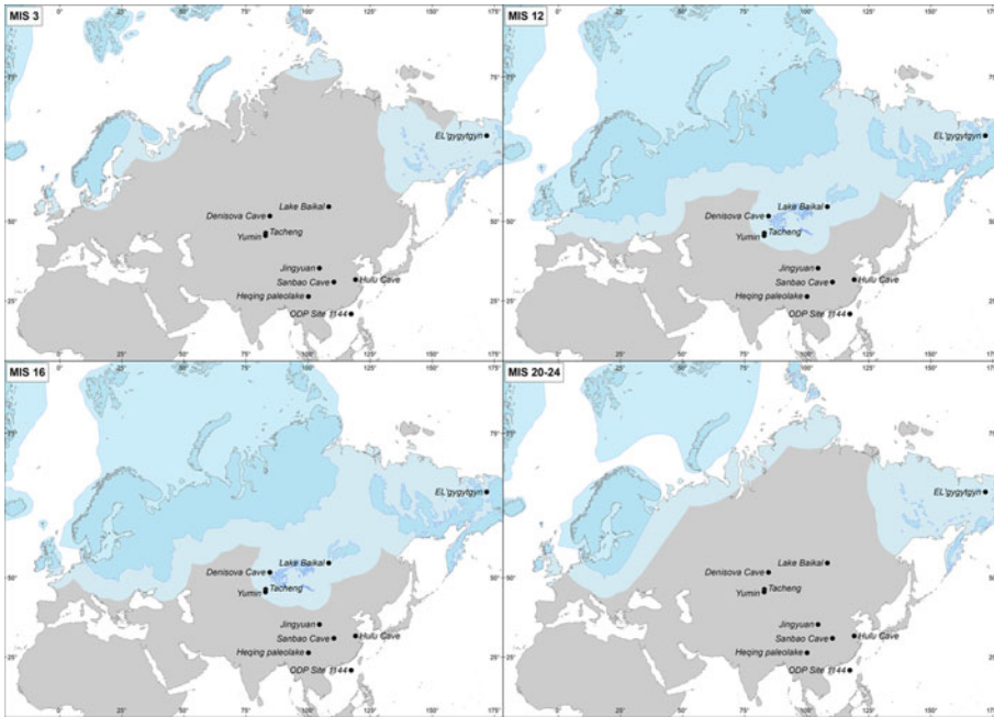
Figure 6. Reconstructed ice-sheet expansion (dark blue) during MIS 24–20 (928–790 ka), MIS 16 (650 ka), MIS 12 (450 ka) and MIS 3 (45 ka) from (Batchelor et al., 2019) and the associated extension of the permafrost (lighter blue) that is estimated at an average of 550 km extension towards the south based on the permafrost extension during the Last Glacial Maximum in Europe (Lindgren et al., 2016).
