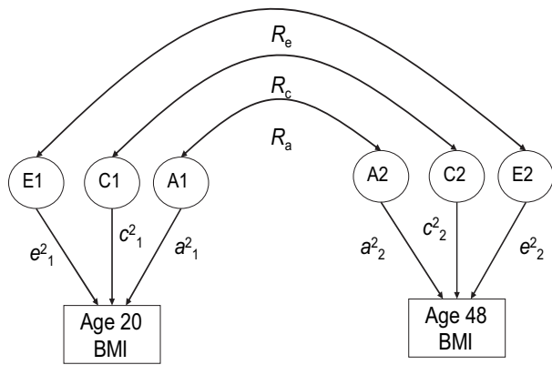
Figure 1 Correlated factors model.
