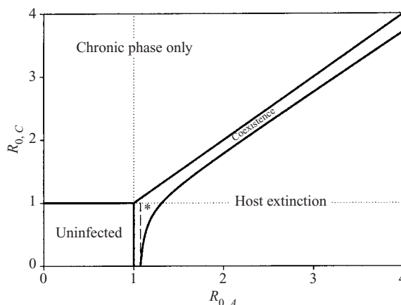
Fig. 2. R_0 map, showing the effects on equilibrium behaviour of varying R_{0,A} and R_{0,C} , by changing \beta_1 and \beta_2 , respectively. There are four modes: uninfected ( R_{0,A}, R_{0,C} < 1 ); chronic phase infection only ( R_{0,C} > 1, R_{0,A} < R_{0,C} ); coexistence:
