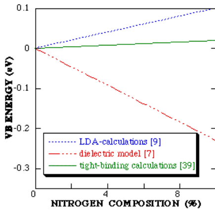
Figure 13. Compositional dependence of the VB edge for strain-free GaNAs predicted by various theoretical calculations. The legend indicates the references.
