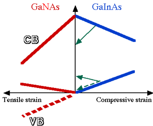
Figure 16. Schematic diagram of band lineup for GaNAs and GaInAs. The use of strain for the horizontal axis allows to demonstrate the effect of nitrogen on the band gap edges [12] (increasing the In content leads to a compressive strain, whereas increasing the N content causes a tensile strain). The arrows show the effect of nitrogen on the CB and VB edges of GaInAs. Dotted line and arrow are related to the theoretical predictions based on the dielectric model. Solid green arrow assumes the N-induced increase in the VB edge of GaInAs, as predicted by the LDA [10] or tight-binding [39] calculations for the GaNAs alloy (shown by solid red line).
