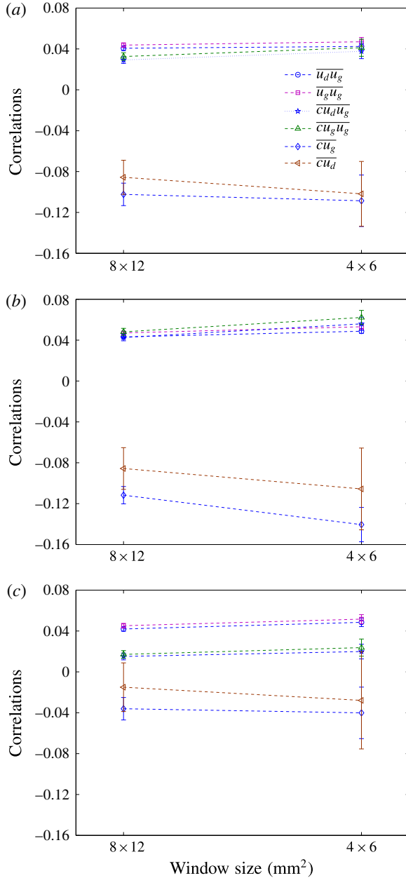
FIGURE 13. (Colour online) Various correlations (corresponding to axial velocity component) appearing in (1.1) for two different window sizes i.e. original measurement window of 8 \times 12 \text{ mm}^2 and window size of 4 \times 6 \text{ mm}^2 with its centre coinciding with the original window for measurement locations, R = 185 \text{ mm} , and for droplet size class of (a) 20\text{--}35 \text{ }\mu\text{m} , (b) 35\text{--}50 \text{ }\mu\text{m} and (c) 50\text{--}65 \text{ }\mu\text{m} .
