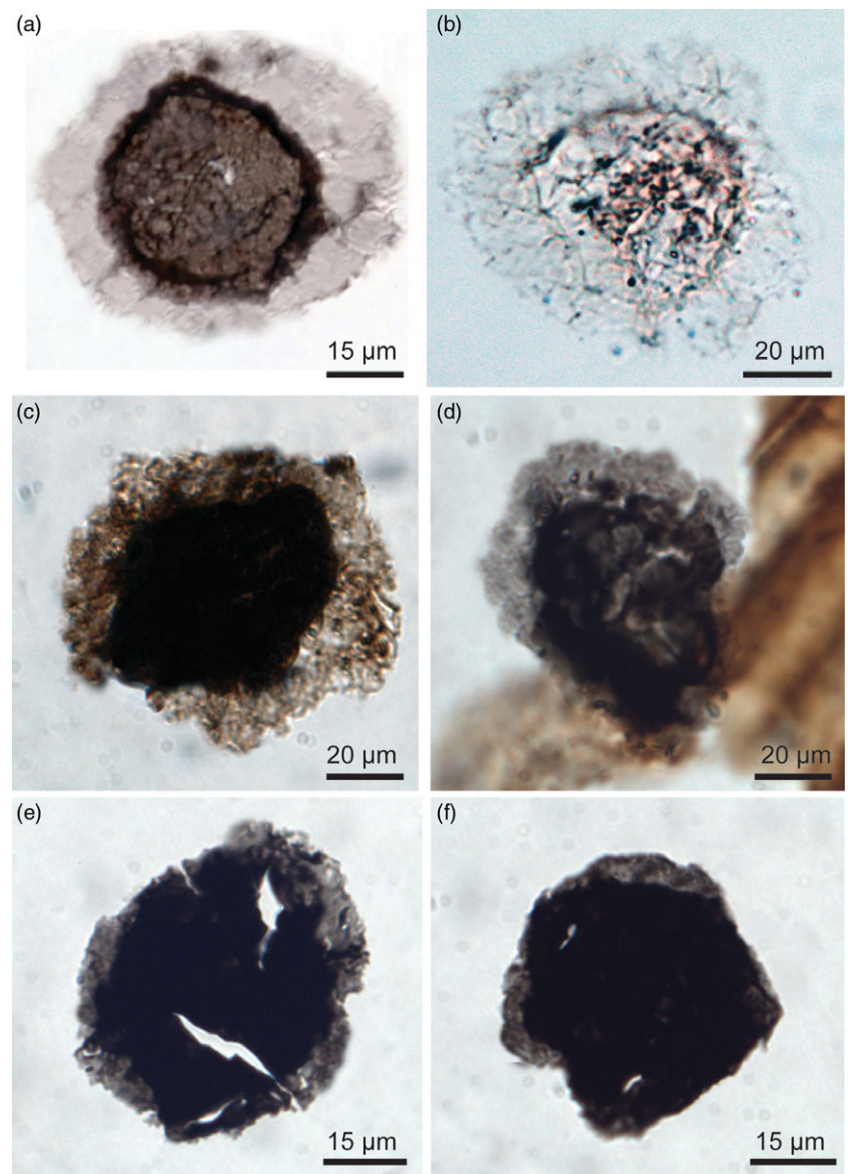
Fig. 4. Transmitted light photomicrographs of the Ediacaran-Cambrian acritarch taxon Granomarginata from various Ediacaran units. (a–d) Granomarginata squamacea . (a) G. squamacea from the Mara Member, Dabis Formation, Nama Group on Farm Pockenbank, Namibia. N16-HA-P2 82×13. (b) N16-HA-P3 81×9, Mara Member. (c) TSGf18448, D18-HA-20 83×16, Indreelva Member, Ståhpogieddi Formation, Vestertana Group on Digermulen Peninsula, Arctic Norway. (d) TSGf18449a, D16-HA-80 87×19, Indreelva Member. (e, f) Granomarginata prima from the Indreelva Member in Norway. (e) TSGf18449b, D16-HA-80 84.5×18. (f) TSGf18450a, D16-HA-53 81×14.
