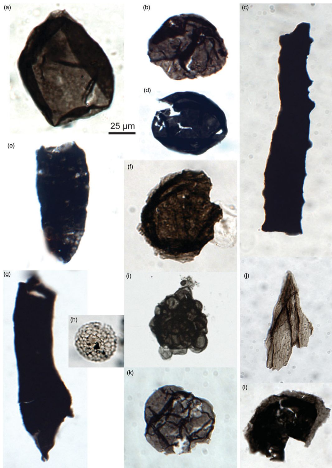
Fig. 6. Other common organic-walled microfossils co-occurring with Granomarginata and Lagoenaforma gen. nov. in units of middle–late Ediacaran age, common components of the late Ediacaran leiosphaerid palynoflora (LELP, cf. Grey, 2005) as well as older Precambrian assemblages, and small carbonaceous fossils. (a) Leiosphaeridia jacutica from the upper Mara Member, Dabis Formation, Nama Group on Farm Pockenbank, Namibia. N16-HA-P2 78×19. (b) Leiosphaeridia crassa from the Mara Member, N16-HA-P2 89×11. (c) Unnamed Form B, a small carbonaceous problematicum with lateral protrusions, from the Gibbett Hill Formation, Signal Hill Group, Avalon Peninsula, Newfoundland. Brasier Shale A-1 91×11. (d) L. crassa from the Indreelva Member, Ståhpogieddi Formation, Vestertana Group in Norway. TSGf18449d, D16-HA-80 85.5×9. (e) Unnamed Form C, tapering elongated and annulated microfossil from the Indreelva Member. TSGf18450b, D16-HA-53 85×9. (f) Simia annulare from the Mara Member, Dabis Formation, Nama Group in Namibia. N16-HA-P2 77×10. (g) SCF from the Manndrapselva Member, Ståhpogieddi Formation. TSGf18451b, D16-HA-77 88×14. (h) Bavlinella sp. from the Mara Member. N16-HA-P2 80×11. (i) Symplassosphaeridium sp. from the Indreelva Member. TSGf18449e, D16-HA-80 80×18. (j) SCF problematicum from the Mara Member. N16-HA-P2 77×16. (k) Lobate or dividing acritarch, from the Indreelva Member. TSGf18449f, D16-HA-80 81×7. (l) Fragmented microfossil with a spongy envelope, Granomarginata prima from the Gibbett Hill Formation, Newfoundland. Brasier Shale A-1 87×5. Scale bar is the same for all images: 25 μm. All images are transmitted light photomicrographs.
