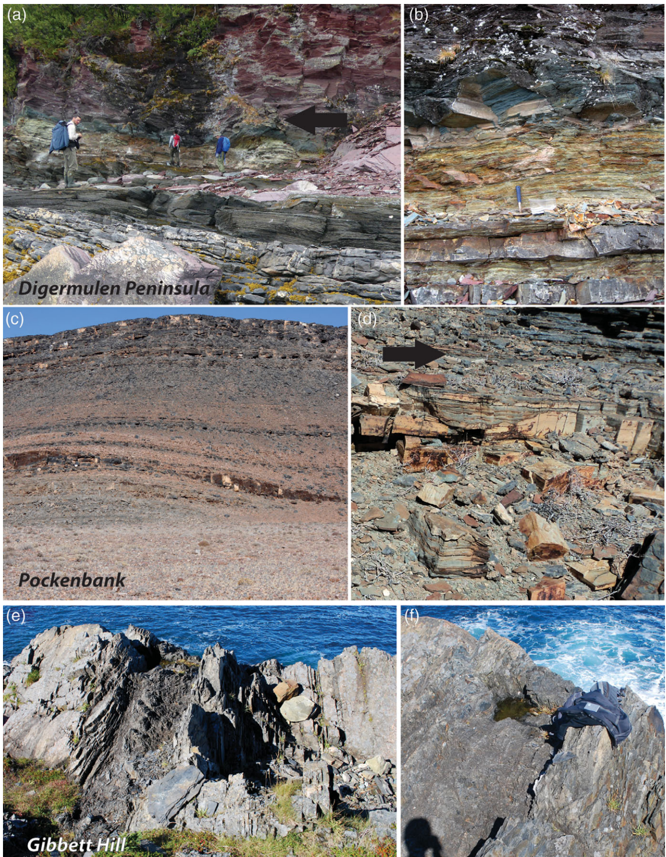
Fig. 1. Localities of sample collections and outcrops with occurrences of Granomarginata and Lagoenaforma gen. nov. (a) Basal part of the Indreelva Member of the Ståhpogieddi Formation, Vestertana Group in coastal outcrops in northern portion of Árasulluokta Cove, southeastern shore of the Digermulen Peninsula in Norway. (b) Shales and siltstones of the Indreelva Member above the occurrence of macrofossil Palaeopascichnus . (c) Basal Nama Group strata on Farm Pockenbank in the Witputs sub-basin in Namibia. (d) Fine arenite of the Mara Member, Dabis Formation, Nama Group exposed on Farm Pockenbank. (e) Gibbett Hill Formation, exposed at the 'Brasier Shale' outcrop on the northern shore of Ferryland Head, eastern coast of the Avalon Peninsula, Newfoundland. This locality was named in honour of Professor Martin Brasier who spent many field excursions studying this outcrop. (f) Enhanced view of the Brasier Shale in the upper Gibbet Hill Formation.
