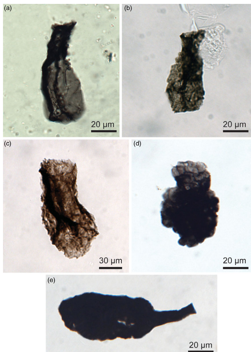
Fig. 5. Transmitted light photomicrographs of the new flask-shaped organic-walled microfossils Lagoenaforma gen. nov. from the middle-upper Ediacaran strata. (a) Lagoenaforma collaris gen. et sp. nov. from the Indreelva Member, Ståhpogieddi Formation, Vestertana Group on Digermulen Peninsula, Norway. (a) Holotype, TSGf18449c, D16-HA-80 78×15. (b, c) L. collaris from the Mara Member, Dabis Formation, Nama Group on Farm Pockenbank in Namibia. (b) N16-HA-P2 76×7. (c) N16-HA-P2 77×5.5. (d) Unnamed Form A, microfossil with a neck-like protrusion from the Manndrapselva Member, Ståhpogieddi Formation, Vestertana Group. TSGf18451a, D16-HA-77 89×23. (e) Opaque neck-bearing microfossil Lagoenaforma sp. from the Gibbett Hill Formation, Signal Hill Group, Avalon Peninsula, Newfoundland. Brasier Shale A-1 87×11.
