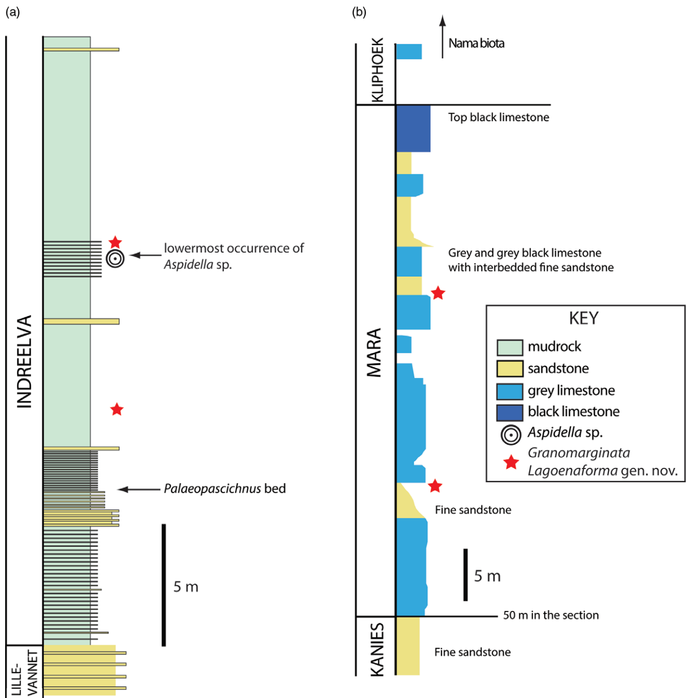
Fig. 3. (a) Microfossil occurrence close to Palaeopascichnus and aspidellomorphs in the lower Indreelva Member, Digermulen Peninsula, Norway. (b) Microfossil occurrence in the Mara Member, Farm Pockenbank, Namibia.
