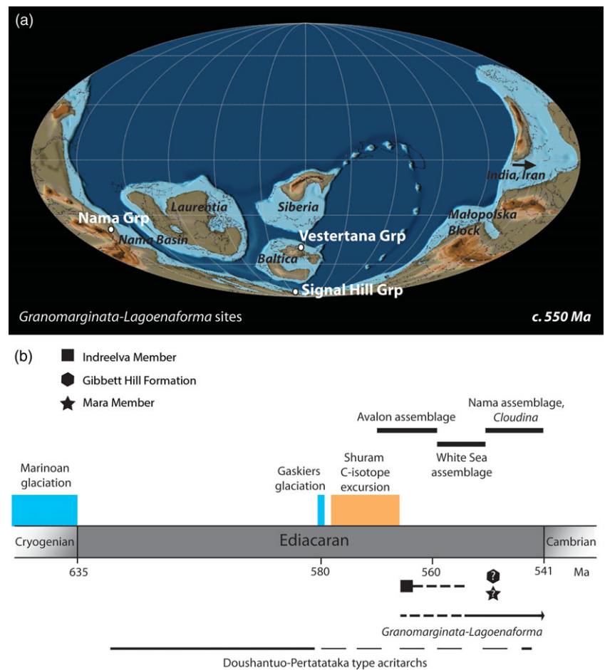
Fig. 7. Distribution and occurrences of documented Granomarginata-Lagoenaforma in the Ediacaran Period. (a) Microfossils from the studied units occur in three distinct areas: Baltica (Indreelva Member, Vestertana Group), Avalonia (Gibbett Hill Formation, Signal Hill Group) and Nama Basin (Mara Member, Nama Group), in white. Localities with additional occurrences of Ediacaran Granomarginata or flask-shaped organic-walled microfossils are marked in black. Continental reconstruction around 550 Ma was produced using PaleoAtlas for GPlates program (Scotese, 2016). (b) Schematic timeline of the appearance and the stratigraphic range of Granomarginata-Lagoenaforma relative to macrofossil assemblages and major environmental events in the Ediacaran Period. The orange box represents the permissible time of the duration of the Shuram negative carbon isotope excursion, following Rooney et al. (2020). Fossiliferous localities are marked by black symbols. A dashed line represents the interval of age-uncertainty for each locality (see Discussion for details).
