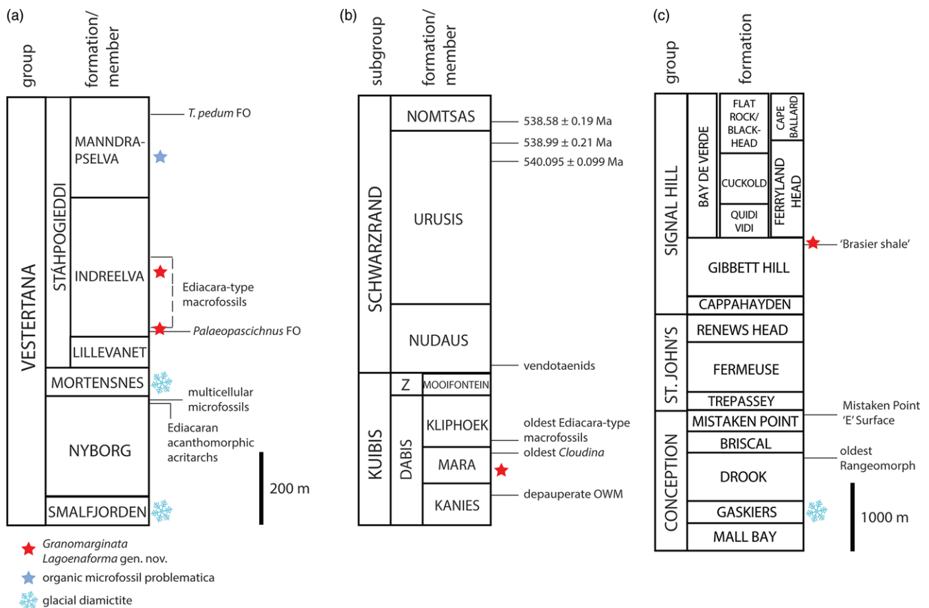
Fig. 2. Simplified schematic regional stratigraphy of the units from which Granomarginata and Lagoenaforma microfossils were recovered, showing the occurrence of microfossils in relation to the Ediacara-type biota and other stratigraphic markers. Stratigraphic markers from each unit are included to inform about the broad age-range of Granomarginata – Lagoenaforma . (a) Ediacaran part of the Vestertana Group exposed on the Digermulen Peninsula in Arctic Norway. The Ediacaran–Cambrian boundary is in the upper part of the Manndrapselva Member, indicated by the first occurrence (FO) of Treptichnus pedum . For the distribution of palaeopascichnids and trace fossils in the Vestertana Group see Jensen et al. (2018b). (b) Stratigraphy of the Nama Group in the Witputs sub-basin, Namibia, modified from Hall et al. (2013). Previous record of depauperate microfossils from Germs et al. (1986). U–Pb zircon age constraints in the Spitzkopf Member, Urusis Formation from Linnemann et al. (2019). (c) Stratigraphy of the Conception, St John's and Signal Hill Groups, based on King (1988) and Matthews et al. (2021). The stratigraphic position of the 'Brasier Shale' outcrop at Ferryland Head is indicated.
