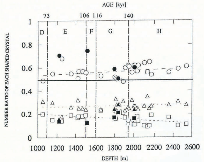
Fig. 3. Depth profiles of the number ratio of three types of air-hydrates in the Vostok ice core: spherical crystal, Ns/N (circle); irregular one, Ni/N (square) and faceted one, Nf/N (triangle). The data of the A series are shown by solid symbols and those of the B series by open symbols. The climatic stages D–H are from Lorius and others (1985).
