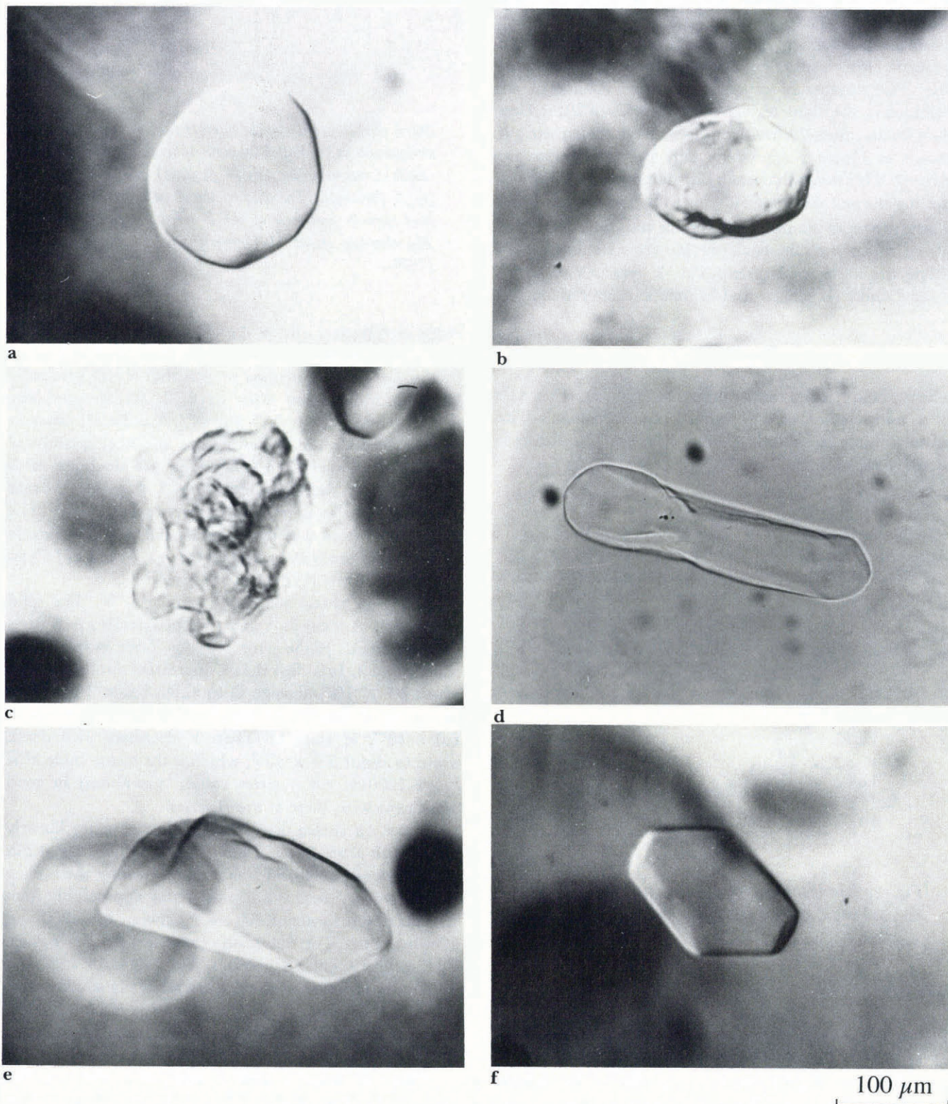
Fig. 1. Air-hydrate crystals observed in ice cores from Vostok: (a) spherical; (b) oval; (c) irregular; (d) rod-like; (e) crystals which had facets; (f) polyhedral. The bar is 100 \mu\text{m} long.
