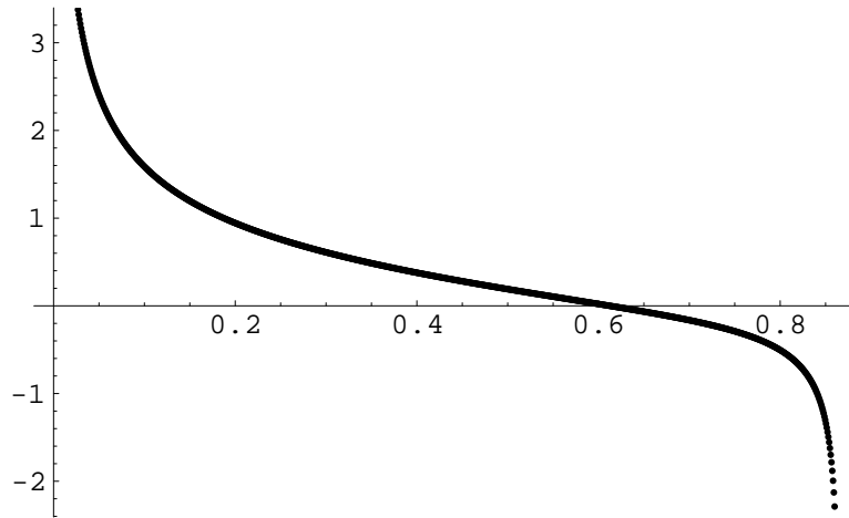
Figure 1: Graph of \cot(\alpha(p)) for 0 < p < \sqrt{3}/2 . The only zero occurs for p = \sqrt{\frac{3}{8}} \approx 0.612 .
