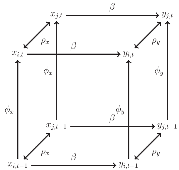
FIGURE 5. Space-Time Dependence
