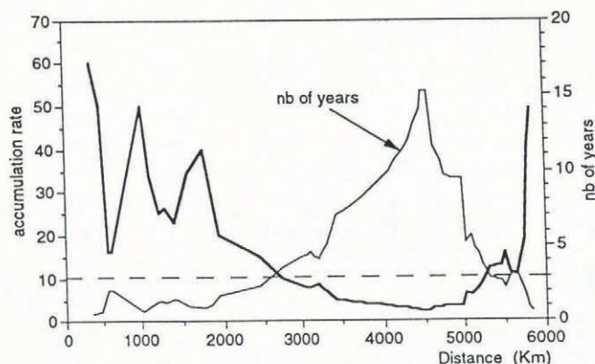
Fig. 3. Estimated accumulation rate ( g\text{ cm}^{-2}\text{ a}^{-1} ) and number of years represented by the 1 m of snow sampled along the traverse route. The horizontal line corresponds to a 3 year snow sequence.
