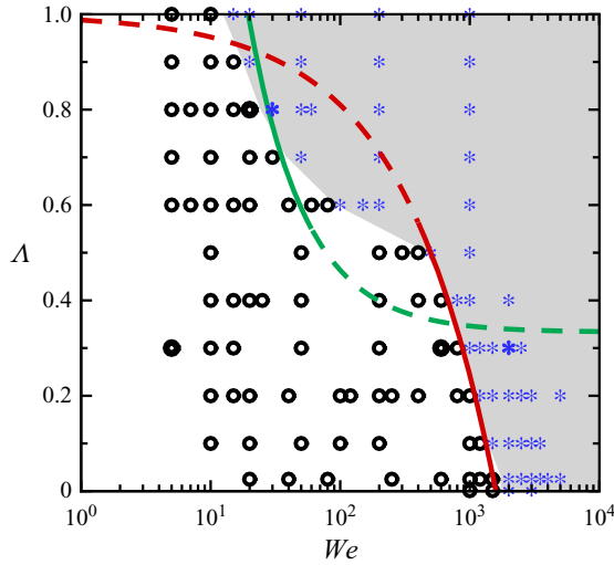
Figure 7. Phase diagram in the We-\Delta parameter space. Empty circles denote the non-breakup regime and stars the interface breakup regime. Symbols with boldface are the cases shown in figures 3 and 5. The grey shadow is a guide to the eye. The red and green lines denote the criteria, (4.3) with prefactor 1590 and (4.6) with prefactor 13.3, for the first and second type of interface breakup, respectively. The solid parts of the lines, where the theory is supposed to hold, indeed nicely agree with the numerical results.
