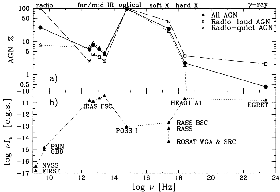
Figure 1. a) (top) The percentage of AGN with detections in a given band vs. frequency for all objects ( solid points ), radio-loud ( open squares ), and radio-quiet ( open triangles ) AGN. Sources without radio data are included in the latter class. b) (bottom) The sensitivity of the deepest all-sky (or very large area) surveys as a function of frequency. The
