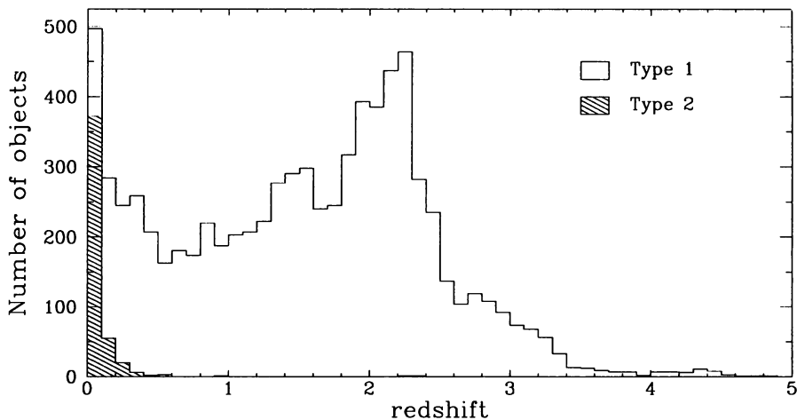
Figure 2. The redshift distribution of the \sim 8,000 radio-quiet AGN in the Véron-Cetty & Véron catalog for Type 1 (broad-lined) and Type 2 (narrow-lined) objects. Only 3 Type 2 radio-quiet AGN are known at z > 0.9 .
