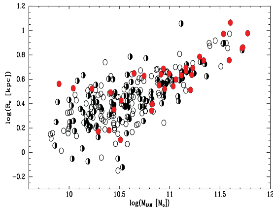
Figure 2. Effective radius, R_e^{\text{max}} , vs M_{\text{JAM}} , a proxy of the stellar mass, for the full sample of ATLAS 3D ETGs (open circles, Cappellari et al. , 2012). The galaxies shown with the half filled circles have already deep MegaCam images available from either the ATLAS 3D or NGVS surveys. The images for the other galaxies will be obtained as part of the MATLAS CFHT Large Programme. Those that have a high fine structure index, i.e. galaxies that are either strongly tidally perturbed, or have multiple stellar streams in their vicinity, are shown with the red filled circles.
