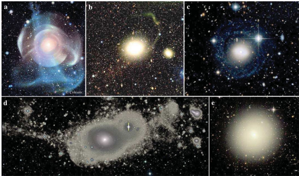
Figure 1. Deep optical images of a sub-sample of nearby Early-Type Galaxies obtained with MegaCam on the CFHT as part of the ATLAS 3D and Next Generation Virgo Cluster Survey. The figure illustrates the variety of low surface brightness structures that show up around these galaxies: long tidal tails and shells, telling us about past major mergers (a,d); narrow stellar filaments associated with disrupted dwarf satellites, revealing future minor mergers (b); regular low surface brightness star-forming disks (c); extended featureless stellar halos (e).
