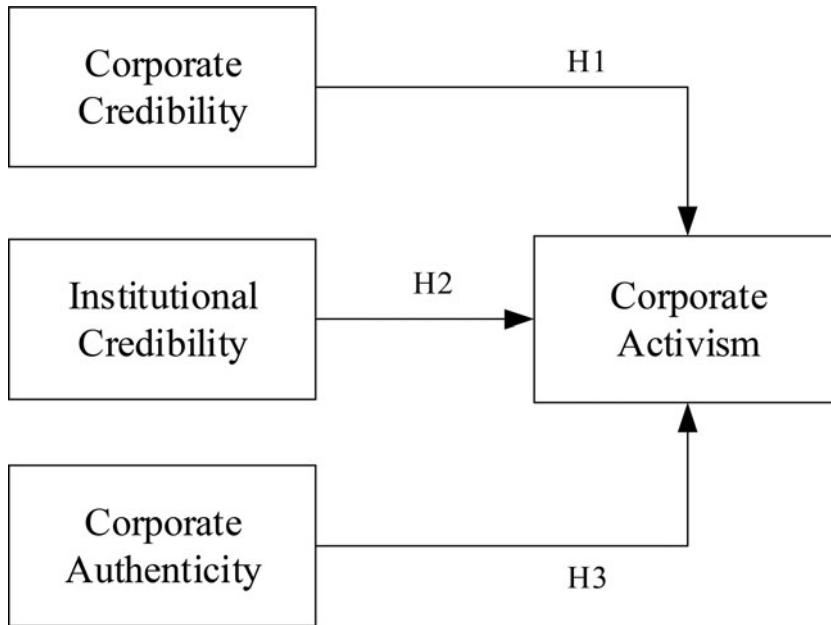
Fig. 1. Conceptual model.
