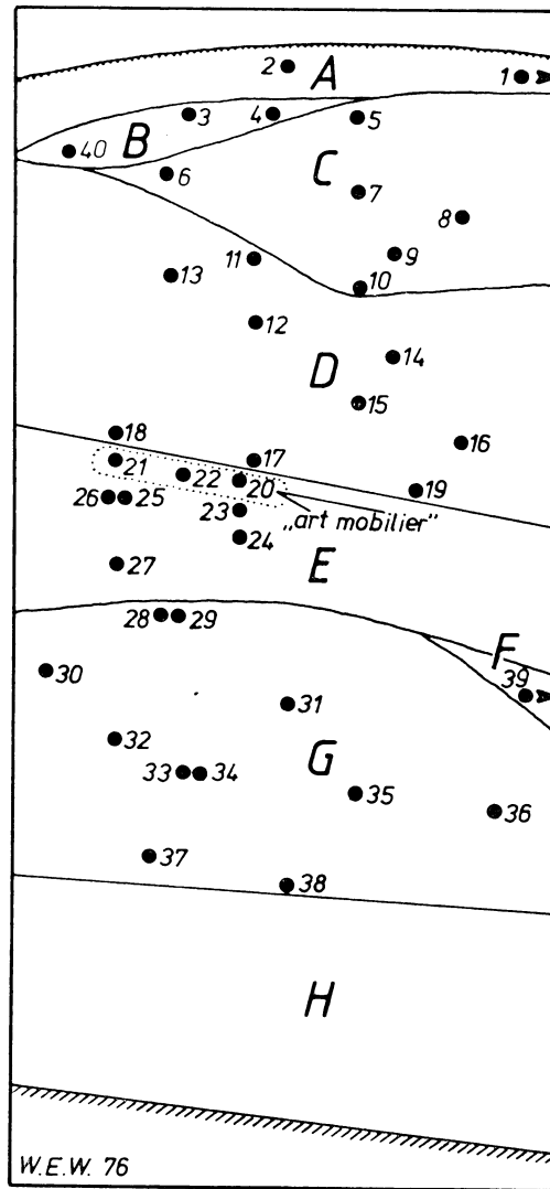
Fig. 1. Apollo 11-Cave: schematic section (not to scale) of main cultural layers, showing positions of all dated ^{14}\text{C} samples listed in Table 2 in relation to each other and to interfaces.
