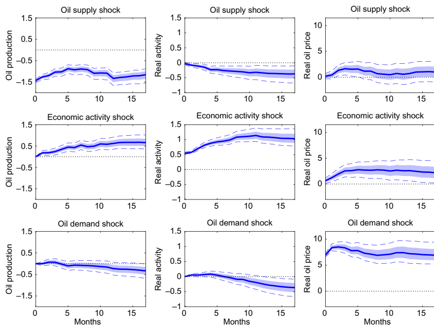
FIGURE 1. Impulse-response functions for three-variable oil market model under traditional Cholesky identification. Solid blue lines: MLE; shaded regions: 68% error bands; dashed blue lines: 95% error bands.
