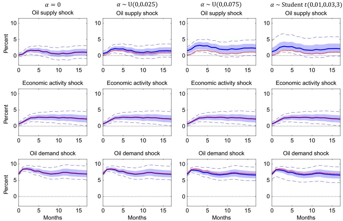
FIGURE 2. Responses of the real price of oil after an oil supply shock, an aggregate demand shock, and an oil-specific demand shock under different priors for the short-run price elasticity of supply as indicated in the header. Dotted red lines: MLEs under Cholesky identification; solid blue lines: median of Bayesian posterior distribution; shaded regions: 68% posterior credibility set; dashed blue lines: 95% posterior credibility set.
