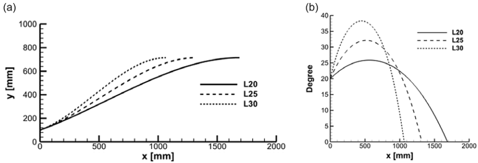
Figure 19. Expansion ramp profile of the LSERN at various lengths with an initial expansion angle of 20°. (a) Expanded ramp profile, (b) Expansion ramp angle.
