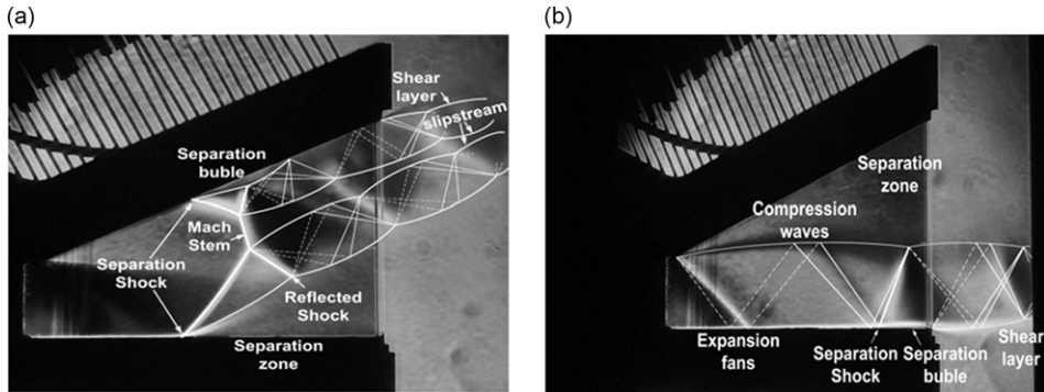
Figure 1. Separation pattern in a straight expansion ramp SERN. (a) RSS (ramp) pattern, (b) RSS (flap) pattern.
