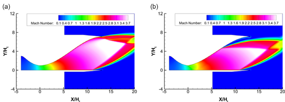
Figure 14. Mach number contours of the flow field inside the nozzle for various initial expansion angles, NPR = 20 . (a) Initial expansion angle of 0^\circ , (b) Initial expansion angle of 10^\circ .
