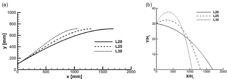
Figure 23. Expansion ramp profile of the LSERN at various lengths with an initial expansion angle of 30^\circ . (a) Expanded ramp profile, (b) Expansion ramp angle.
