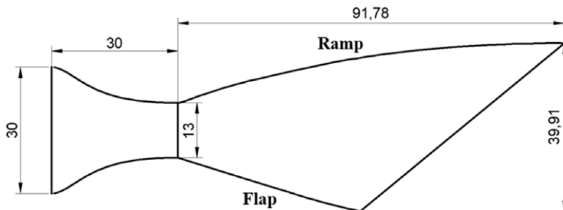
Figure 2. Sketch of the SERN model.
