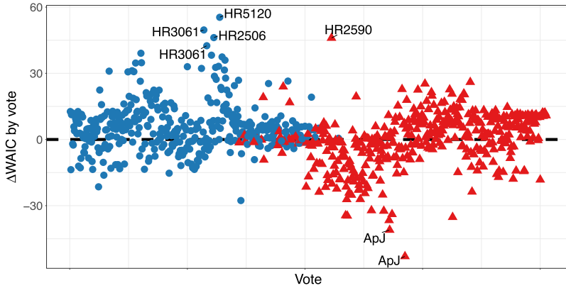
Figure 5. Difference in vote-specific WAIC scores between the probit unfolding model and BGGUM, ( WAIC(BGGUM) - WAIC(PUM) ), for the 107th House. Note that the way the difference is being computed here is the opposite to the way in which it was computed in Figure 3a. Votes are ordered according to the absolute difference between Republican votes and Democratic votes. Blue circles indicate votes in which the voting Democrats’ proportion of “Ayes” is greater than the voting Republicans’ proportion of “Ayes,” whereas red triangles indicate votes in which the reverse happened.
