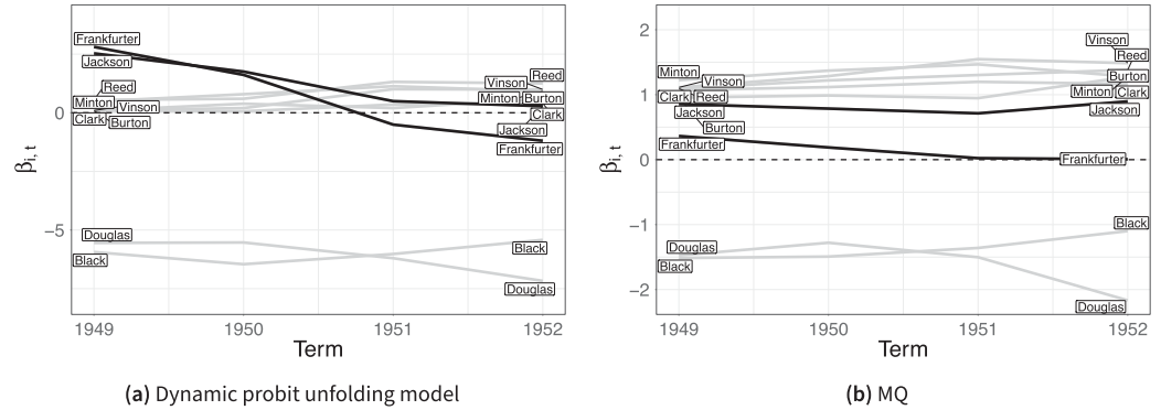
Figure 10. Posterior means of the ideal points for SCOTUS Justices active during 1949–1952 terms under the dynamic unfolding model (left column) and MQ (right column).
