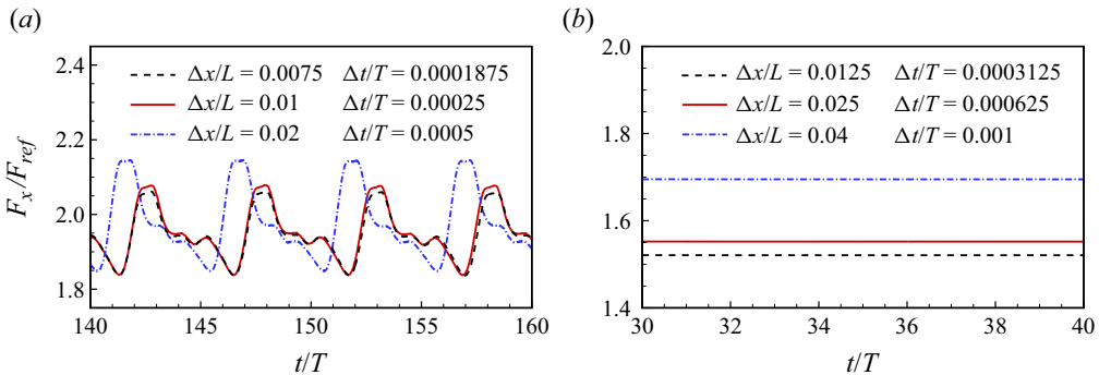
Figure 4. Grid independence and time-step independence study for (a) the 2-D ribbon with M_t = 1 and Re_u = 200 and (b) the 3-D ribbon with M_t = 1 , Re_u = 200 and \mathcal{R} = 0.25 . The streamwise force F_x normalized by F_{ref} = (1/2)\rho U_{ref}^2 L as a function of time is presented.
