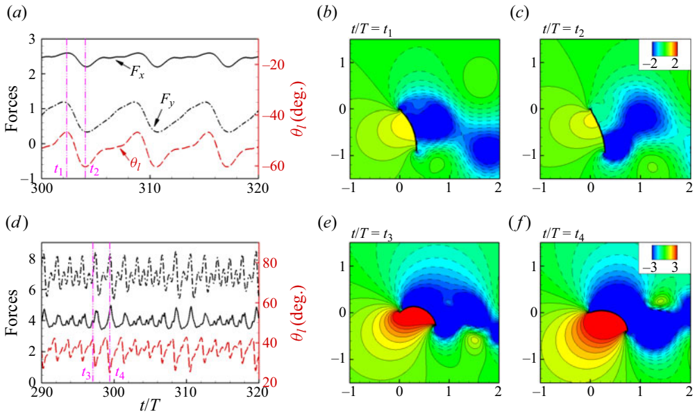
Figure 15. Time history of streamwise force F_x , transverse force F_y and leading edge inclination angle \theta_l for (a) case I: M_f = 2 , Re_u = 200 and (d) case II: M_f = 2 , Re_u = 500 . (b,c) Instantaneous pressure contours in case I. (e,f) Instantaneous pressure contours in case II. At t = t_1 and t_3 , the ribbons reach their maximum \theta_l ; at t = t_2 and t_4 , minimum \theta_l . Solid and dashed lines for pressure contours denote the positive and negative normalized pressure contours.
