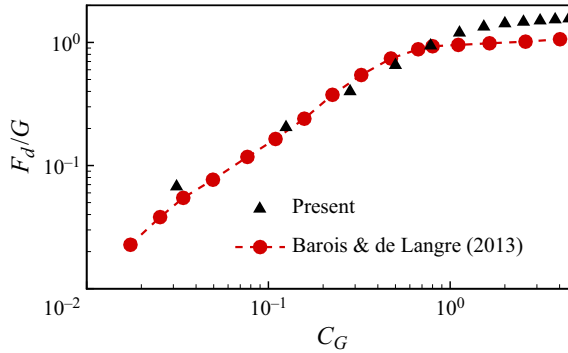
Figure 3. The G -normalized drag F_d/G of the 3-D ribbon as a function of C_G with M_t = 1 and \mathcal{R} = 0.5 . The experimental results of Barois & de Langre (2013) are also presented with \mathcal{R} \approx 0.1 .
