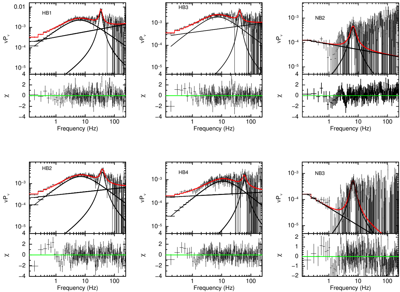
Figure 8. Figure shows the PDS for HID segments HB1, HB2, HB3 HB4, NB2 and NB3 in the energy band 3 – 50 keV. In HB1, HB2 and HB3, a HFO is detected. A NBO is seen in the NB2 and NB3. The PDS for segments HB1, HB2 and HB3 are fitted with the combination of double Lorentzian and a power-law. The PDS for segments NB2 and NB3 are fitted with the combination of a power-law and a Lorentzian. Best fit model along with the observed PDS has been shown in the figure.
