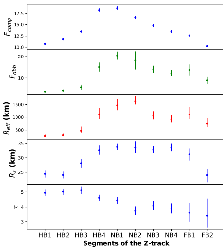
Figure 7. Figure shows evolution of the Comptonized ( F_{Comp} ) flux, disk flux ( F_{dbs} ), the effective inner disk radius ( R_{eff} ) and the optical depth ( \tau ) of the corona, calculated for Model 4 . Significant evolution of the disk and the Comptonized flux is clearly visible. The effective disk radius and optical depth ( \tau ) also evolve significantly from the segment HB1 to FB2. For details see the text and Table 5.
