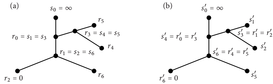
Figure 3: (a) A possible enumeration of edges for the application of Wilson’s method. (b) A possible enumeration of edges for performing the summations using (4.2) in the order j = 1, 2, \dots, 2k . Summing over the spatial location \varphi(s'_j) eliminates the factor involving the edge \{s'_j, r'_j\} . Following this, it is possible to sum over \varphi(s'_2) , etc.
