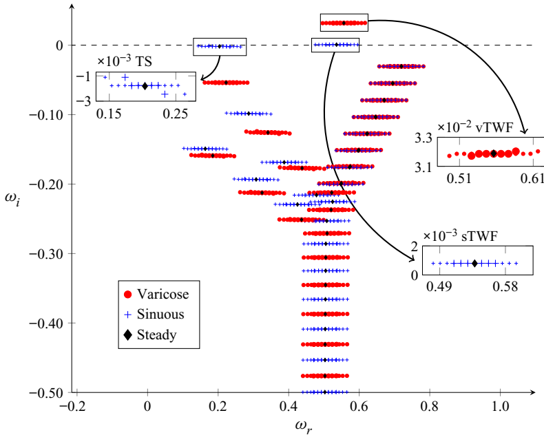
Figure 2. Spectrum for \tilde{Q} = 0.02 , Wo = 10 , V_R = 1 , Re = 10\ 000 , \alpha = 1 , B_* = 4 and d_* = 0 . The steady case corresponds to \tilde{Q} = 0 . In the insets, small symbols correspond to eigenvalues computed with N_f = 6 and large symbols are obtained with N_f = 3 .
