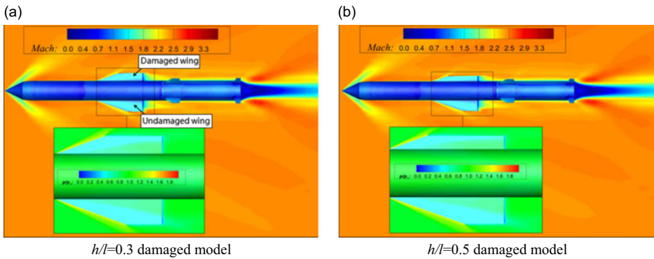
Figure 7. Mach and local pressure contour at \alpha = 4^\circ .
