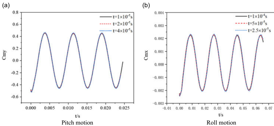
Figure 15. Validation of moment coefficient with time during pith/roll motion (time step independence validation).
