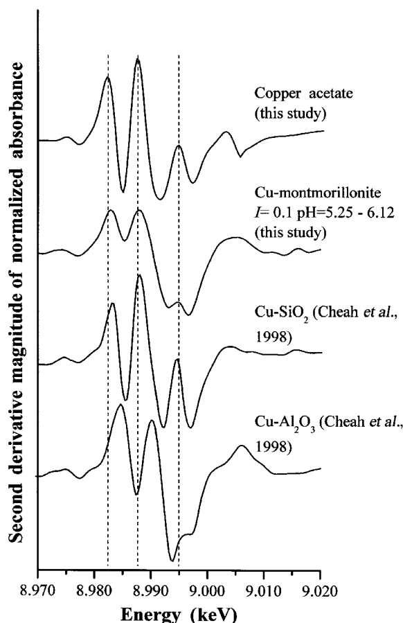
Figure 8. Comparison of second-derivative spectra from montmorillonite samples incubated at high I averaged (see text) with results from Cu sorbed on amorphous SiO 2 and Al 2 O 3 as reported by Cheah et al. (1998). The Cu acetate spectrum was used to correlate the energy of the samples in the two studies.
