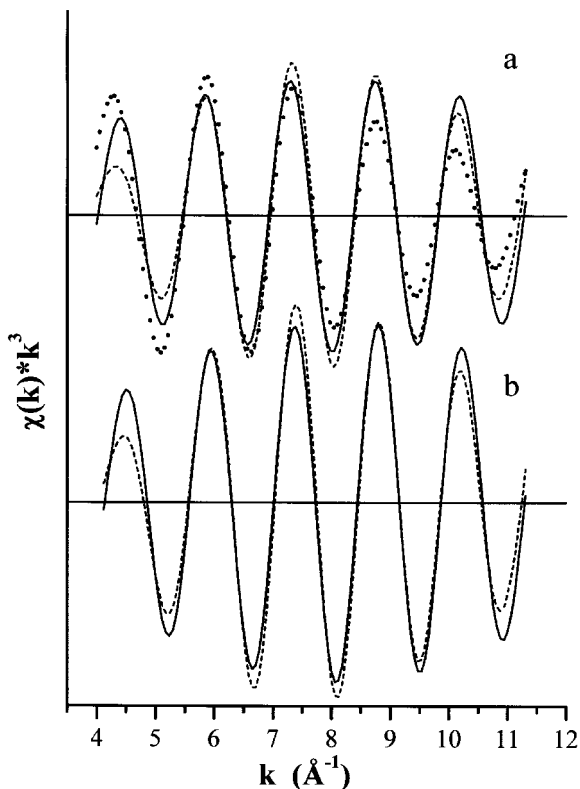
Figure 6. Backtransforms ( \Delta R = 1.9\text{--}2.5 \text{ \AA} ) of (a) second shell in Fourier transform modulus of montmorillonite sample incubated at I = 0.1 \text{ pH} = 6.12 , and (b) Cu acetate sample. The dashed lines are best fits using a single Cu backscatterer atom and the dotted line in panel a is best fit using a single Al backscatterer atom.
