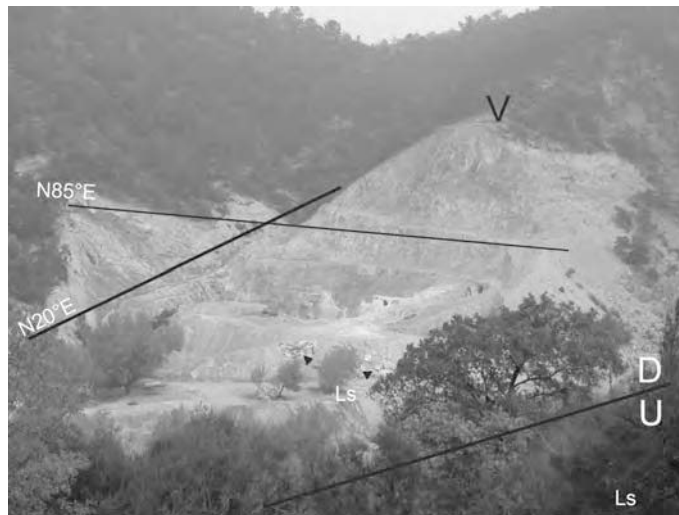
Figure 2. General view of the southern halloysite mine. Hydrothermal mineralization occurred at the intersection of the N20°E (left) and N85°E (right) fault zones. D/U shows the relative displacement of the normal fault. V = volcanics, Ls = limestone terrain.
