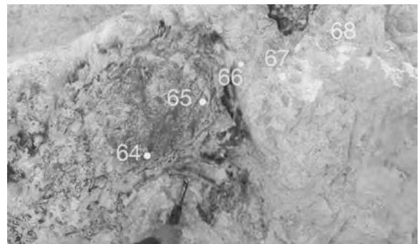
Figure 3. Concentric exfoliation texture of altered andesitic tuffs. Liesegang banding proceeds from the core (T-64) to the most altered region of almost pure halloysite (sample T-68). Corresponding chemical data are given in Table A3, and Figures 4A and 15.
