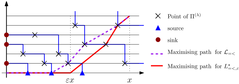
Fig. 5. A sample of \Pi_{x,t}^{(\lambda)} , sources, sinks, and the corresponding trajectories of particles. Here \mathcal{L}_{=<(\Pi_{x,t}^{(\lambda)} \cup \text{So}_x^{(\alpha)} \cup \text{Si}_t^{(p)}) = 5 and L_{=<^{(\alpha,p)}(t) = 2 (two remaining particles at the top of the box).
