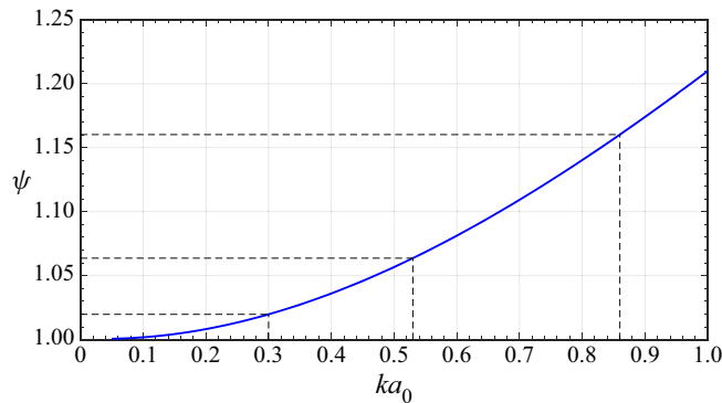
FIGURE 6. Growth reduction factor versus pre-shock ka_0 from the vorticity deposition model of Rikanati et al. (2003) (3.13) for a Mach 1.2 shock travelling from air to SF 6 .
