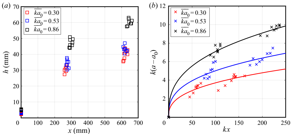
FIGURE 4. (a) Effect of initial conditions on mixing widths with respect to downstream distance. Mean values at x \approx 280 mm are h (mm) = 31.3, 34.2, 47.1 and at x \approx 630 mm are h (mm) = 39.7, 43.3, 60.1 for \overline{ka_0} = 0.30, 0.53 and 0.86 (see table 1 for details). (b) Dimensionless amplitude as a function of normalized distance. Power-law fits follow k(a - a_0) \propto (kx)^n where n = 0.37, 0.35, 0.36 , respectively.
