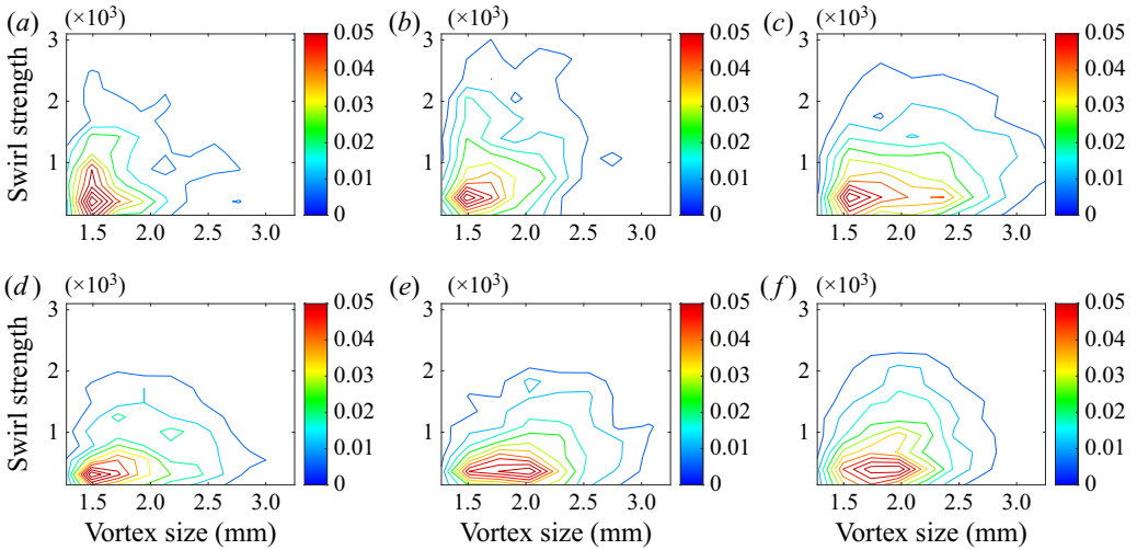
FIGURE 10. Joint probability distribution of vortex size with swirl strength for \overline{ka_0} = 0.30, 0.53 and 0.86 at t = 2.65 ms ( a-c ) and t = 5.65 ms ( d-f ), respectively.
