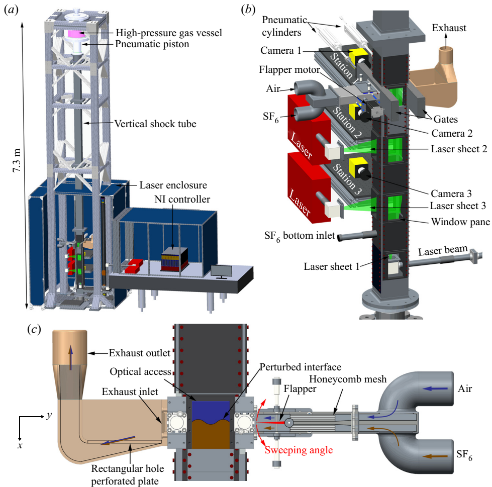
FIGURE 1. Schematic of the experimental set-up. (a) Overview of the 7 m tall vertical shock tube (VST). The shock is generated downwards by a pneumatic piston situated at the top end. (b) Optical diagnostics at stations 1–3 numbered in shock travel direction. Station 1 particle image velocimetry laser sheet is produced vertically from the base of the VST while those for station 2 and 3 traverse horizontally. (c) Close-up overview of the initial condition interface set-up at station 1. Flapper oscillations produce a perturbed interface.
