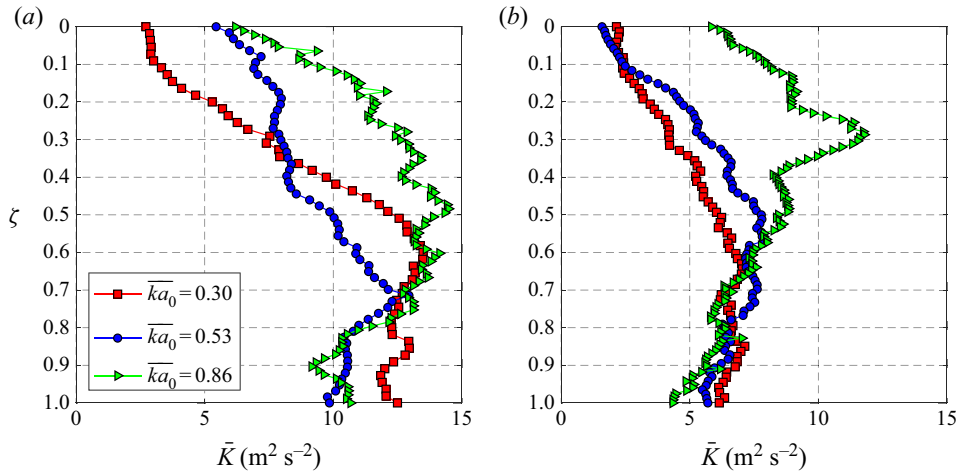
FIGURE 13. Two-dimensional TKE from (3.26) versus the normalized streamwise distance \zeta = x/h for \overline{ka_0} = 0.30, 0.53 and 0.86 at (a) t = 2.65 ms and (b) t = 5.65 ms.
