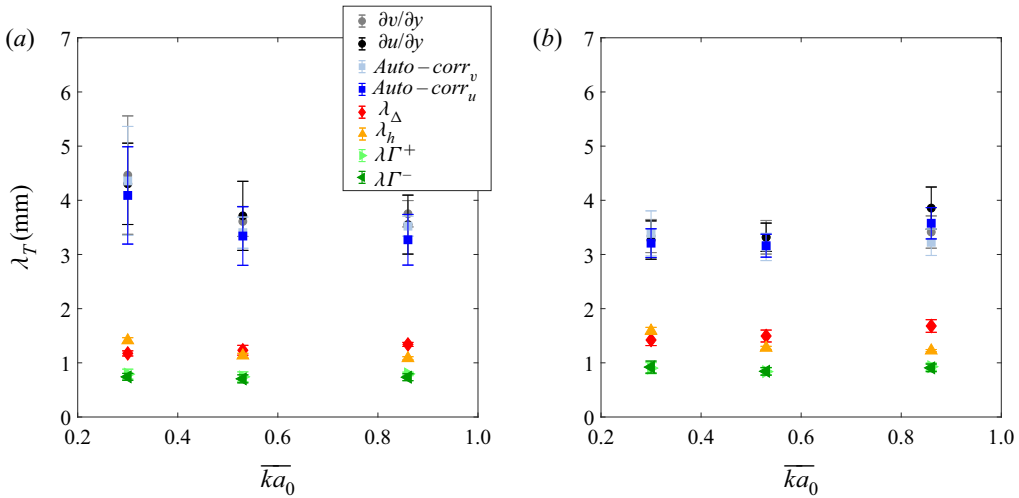
FIGURE 15. Comparison of Taylor micro-scales obtained using spatial gradient ( \partial v/\partial y , \partial u/\partial y ) and autocorrelation ( corr_v , corr_u ) methods with Reynolds number based derivatives ( \lambda_\Delta , \lambda_h , \lambda\Gamma^+ , \lambda\Gamma^- ) from \lambda_T \approx 10hRe^{-1/2} at (a) t = 2.65 ms and (b) t = 5.65 ms.
