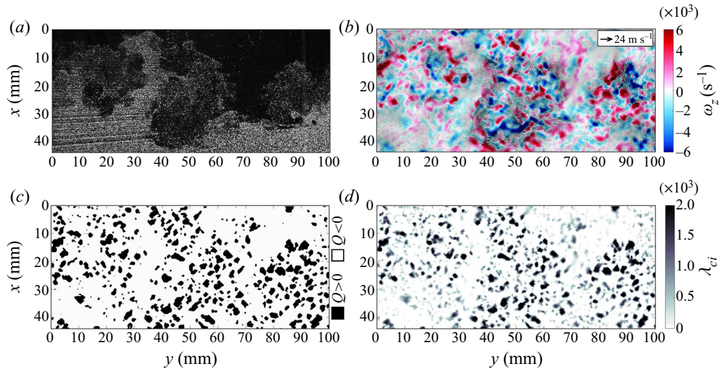
FIGURE 8. (a) PIV image of the mixing width from example shown in figure 2 (c, t = 2.65 ms) and corresponding plots for (b) vorticity, \omega_z , overlaid with velocity fluctuation vectors, (c) Q -criterion and (d) swirl strength, \lambda_{ci} .
