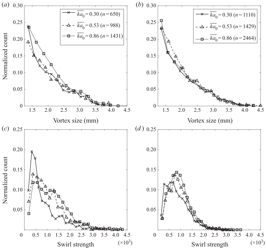
FIGURE 9. Probability distribution of vortex size and swirl strength at t = 2.65 ms ( a,c ) and 5.65 ms ( b,d ) for increasing ka_0 initial conditions. Counts are normalized with respect to total count ( n ).
