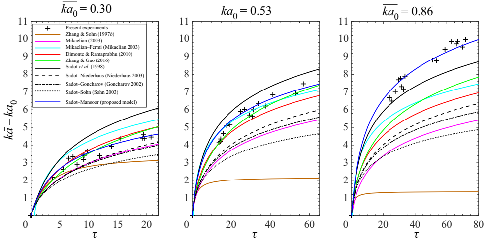
FIGURE 7. Evolution of dimensionless overall amplitude ( k\bar{a} - ka_0 ) versus dimensionless time \tau found in present experiments in comparison with past nonlinear models based on heuristic/interpolation methods (Sadot et al. 1998; Mikaelian 2003), Padé approximation approach (Zhang & Sohn 1997b) and simulations (Dimonte & Ramaprabhu 2010). Asymptotic components are E_{b/s} = \frac{3}{2} \frac{(1 \pm A)}{(1 + A)} (solid black line); E_{b/s} = 1 \pm A (black dashed line); E_{b/s} = \frac{3}{3 \pm A} \frac{(1 \pm A)}{(1 + A)} (black dash-dotted line); E_{b/s} = \frac{(2 \pm A)}{2} (black dotted line); and E_{b/s} = \ln\left(\frac{3}{k\bar{a}_0}\right) \frac{(1 \pm A)}{(1 + A)} (blue solid line).
