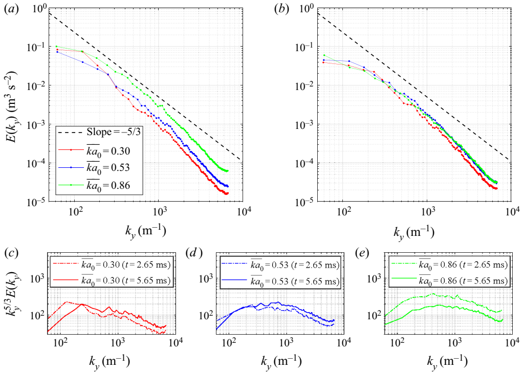
FIGURE 16. Energy spectra for \overline{ka_0} = 0.30, 0.53 and 0.86 at (a) t = 2.65 ms and (b) t = 5.65 ms. Compensated spectra for \overline{ka_0} = 0.30 (c), 0.53 (d) and 0.86 (e) at both times.
