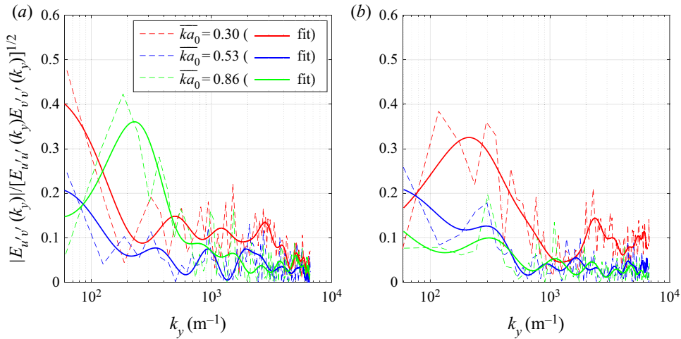
FIGURE 17. Normalized cross-correlation spectrum for \overline{ka_0} = 0.30, 0.53 and 0.86 at (a) t = 2.65 ms and (b) t = 5.65 ms.
