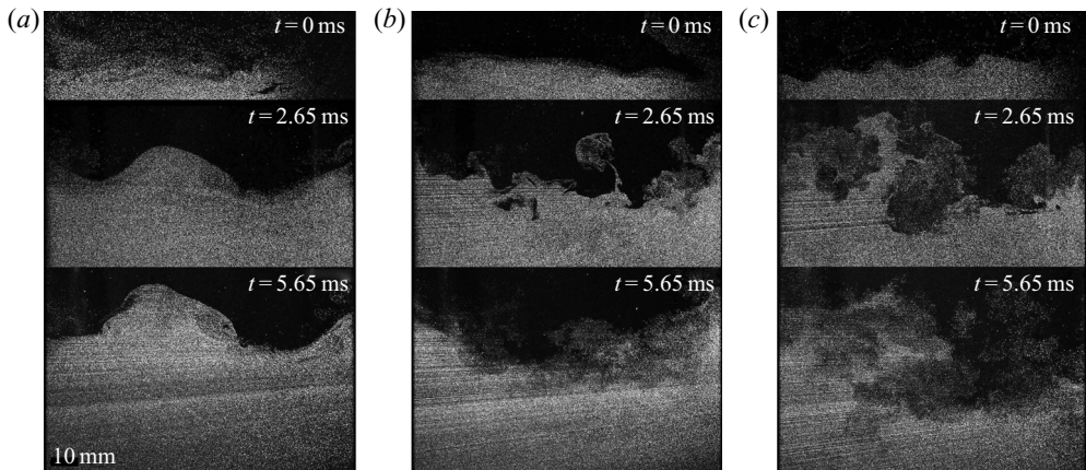
FIGURE 2. Initial condition ( t = 0 ms) and ensuing structures at t = 2.65 and 5.65 ms for \overline{ka_0} = (a) 0.3, (b) 0.53 and (c) 0.86. The cross-flow direction in the initial conditions is from right to left.
