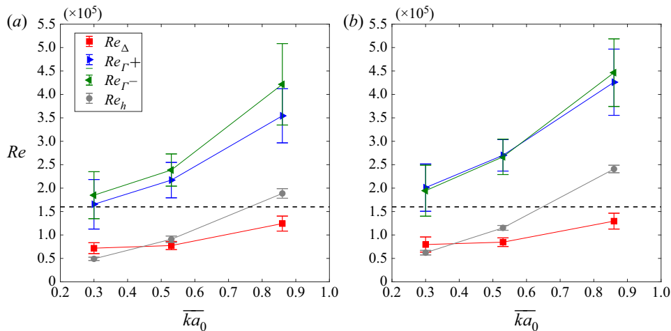
FIGURE 14. Local and global information based Reynolds numbers, Re_\Delta = f(u', h, v) , Re_\Gamma = f(\Gamma, v) and Re_h = f(\dot{h}, h, v) , versus \overline{ka_0} at (a) t = 2.65 ms and (b) t = 5.65 ms. The dashed lines indicate the minimum state criterion of Re = 1.6 \times 10^5 by Zhou (2007).
