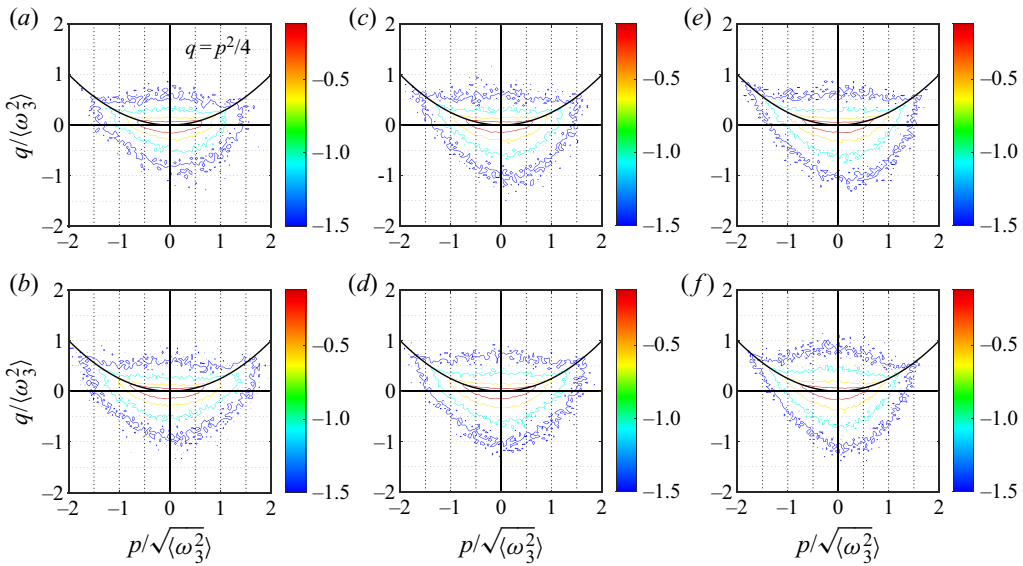
FIGURE 11. Normalized joint p.d.f.s of reduced VGT invariants p and q for ka_0 = 0.30, 0.53 and 0.86 at 2.65 ms ( a, c, e ) and 5.65 ms ( b, d, f ), respectively. Contour levels scale logarithmically. \langle pq \rangle / \langle \omega_3^2 \rangle^{3/2} = (a) -0.053, (b) -0.029, (c) -0.062, (d) -0.029, (e) -0.065, (f) -0.054 . \omega_3 = (\partial u_2 / \partial x_1) - (\partial u_1 / \partial x_2) .
