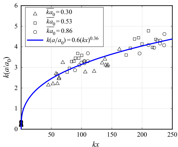
FIGURE 5. Dimensional scaling k(a/a_0) = 0.6(kx)^{0.36} yields minimum scatter for present data.
