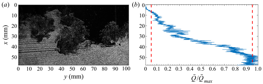
FIGURE 3. Normalized mean concentration distribution of olive oil particles with streamwise distance; \bar{Q}_{max} represents the maximum of the mean concentration profile. The dashed lines indicate 5% and 95% of the mean particle concentration ( \overline{ka_0} = 0.86 , t = 2.65 ms, h = 44 mm).
