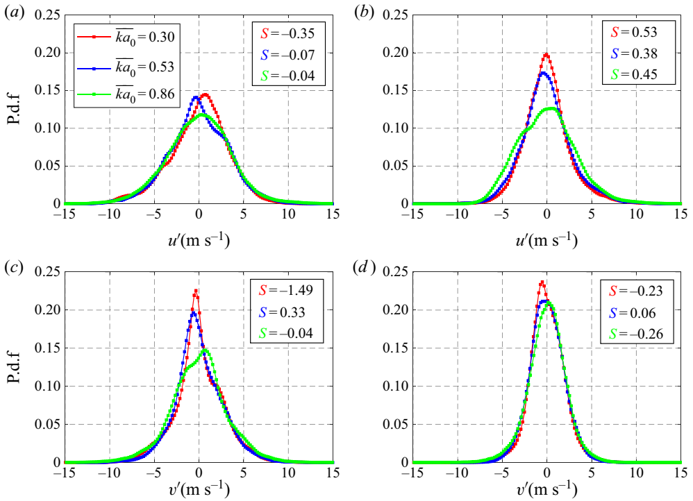
FIGURE 12. Probability density functions of (a,b) streamwise, u' and (c,d) spanwise velocity fluctuations v' at t = 2.65 ms (a,c) and t = 5.65 ms (b,d) for \overline{ka_0} = 0.30, 0.53 and 0.86 . S represents skewness.
