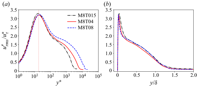
Figure 4. The normalised turbulent intensity of the streamwise velocity u''_{rms}/u^*_\tau plotted against (a) semilocal scaling ( y^* ) and (b) outer scaling ( y/\delta ). The vertical dashed line represents y^* = 18 in (a).
