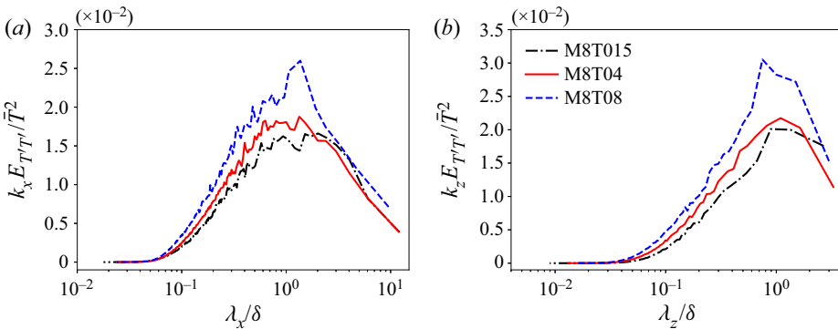
Figure 30. (a) The normalised premultiplied streamwise spectra of the fluctuating temperature k_x E_{T'T'} / \bar{T}^2 at y/\delta = 0.8 plotted against \lambda_x / \delta . (b) The normalised premultiplied spanwise spectra of the fluctuating temperature k_z E_{T'T'} / \bar{T}^2 at y/\delta = 0.8 plotted against \lambda_z / \delta .
