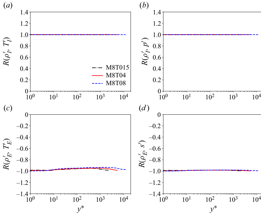
Figure 7. The correlation coefficients (a) R(\rho'_1, T'_1) , (b) R(\rho'_1, p') , (c) R(\rho'_E, T'_E) and (d) R(\rho'_E, s') along the wall-normal direction plotted against semilocal scaling ( y^* ).
