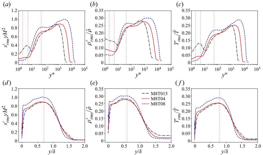
Figure 6. (a,d) The normalised turbulent intensity of the entropy s'_{rms}\gamma M^2 along the wall-normal direction against (a) semilocal scaling ( y^* ) and (d) outer scaling ( y/\delta ). The vertical dashed lines represent y^* = 2, 5, 50 in (a) and y/\delta = 0.7 in (d), respectively. (b,e) The normalised turbulent intensity of the density \rho'_{rms}/\bar{\rho} along the wall-normal direction against (b) semilocal scaling ( y^* ) and (e) outer scaling ( y/\delta ). The vertical dashed lines represent y^* = 2, 5, 40 in (b) and y/\delta = 0.6 in (e), respectively. (c,f) The normalised turbulent intensity of the temperature T'_{rms}/\bar{T} along the wall-normal direction against (c) semilocal scaling ( y^* ) and (f) outer scaling ( y/\delta ). The vertical dashed lines represent y^* = 2, 5, 50 in (c) and y/\delta = 0.8 in (f), respectively.
