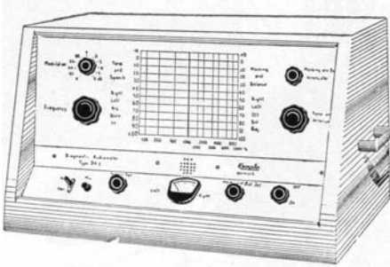
CLINIC AUDIOMETER DA1
