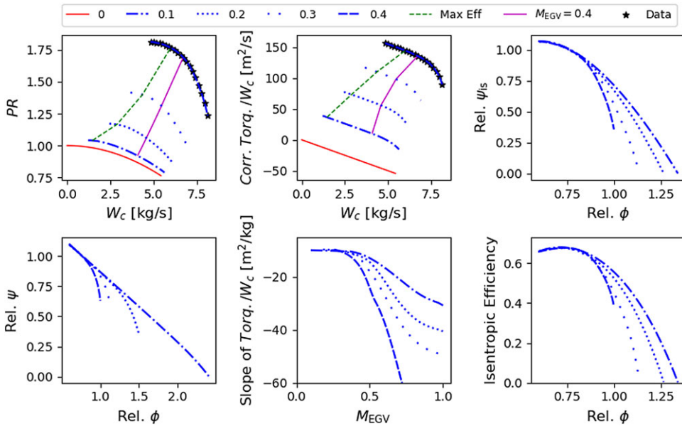
Figure 2. A compressor sub-idle map extended using the above-explained methodology.
