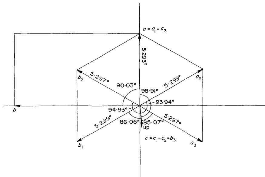
Fig. 1. Unit cells for talc. Axes without subscripts are for the C cell. Subscripts are for the three P cells (see Table 2).
