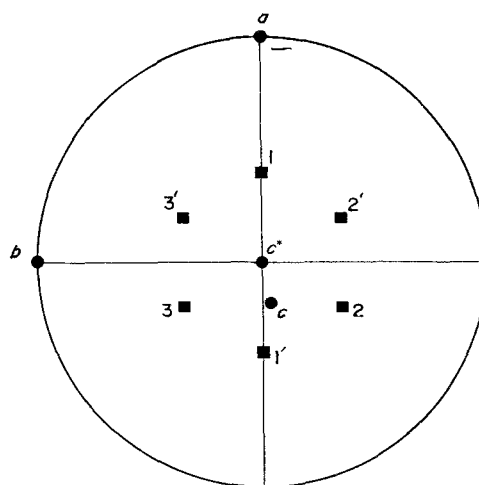
Fig. 2. The relationship of the six trial structures of talc to the crystal axes. The cell axes (●) and the six possible orientations of the layer represented by the shortest vector from lower to upper OH groups (■).
