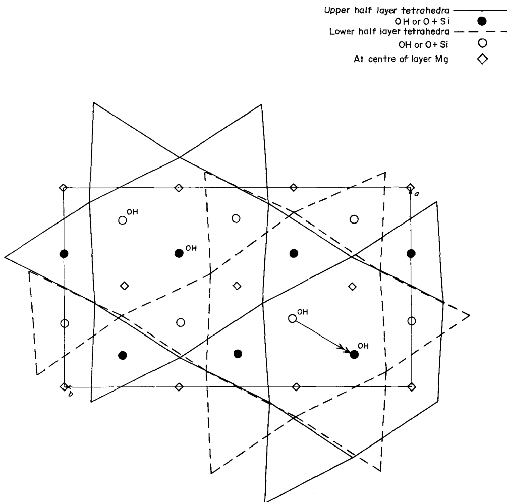
Fig. 3. Projection of a single layer of the talc structure perpendicular to the layer. The bases of the tetrahedra are outlined with continuous lines at the top of the layer ( z = 0.35 ) and with pecked lines at the bottom ( z = -0.35 ). Octahedral O and OH are shown as ● at z = 0.12 and at ○ at z = -0.12 and magnesium at the centre ( z = 0 ) as ◇. The double headed arrow is the shortest OH-OH distance and this vector is used to show the orientation of the layers in Fig. 2.
