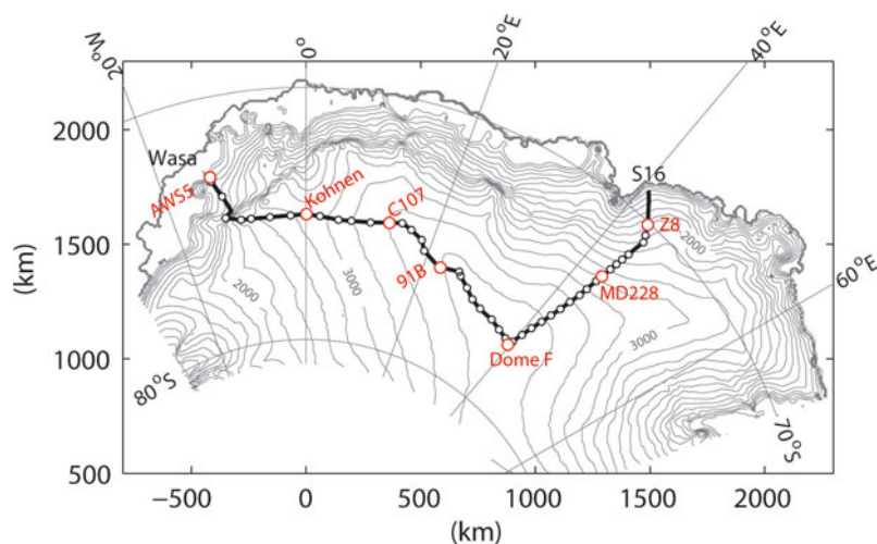
Fig. 1. Map of the study region, along with the route traversed by the Japanese–Swedish Antarctic Expedition in 2007/08. Open circles denote the locations of snow-pit measurements. Red circles denote measurement sites referred to in the text. The contours represent surface elevation at intervals of 200 m, based on Bamber and others (2009).
