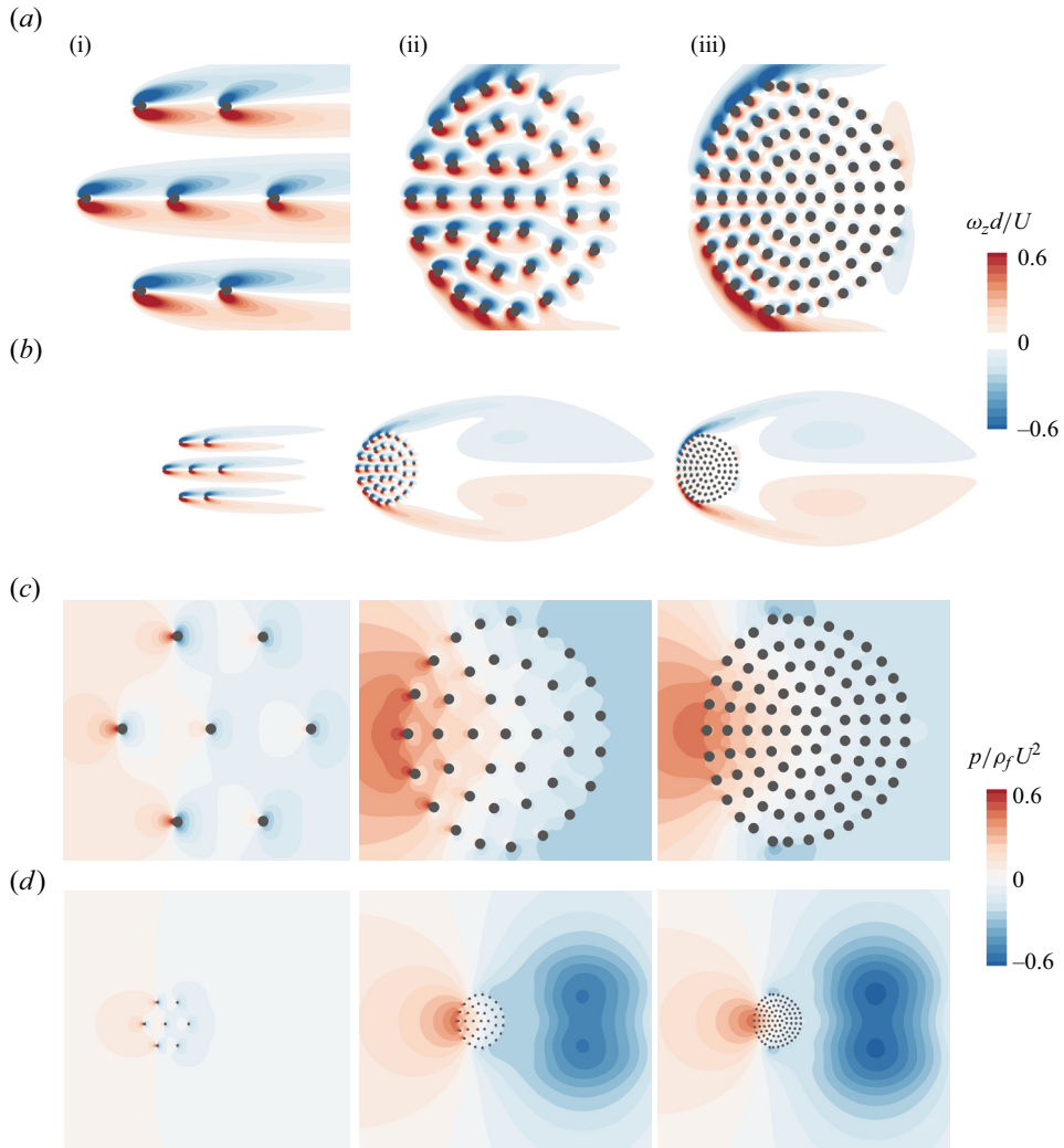
Figure 10. (a,b) Vorticity and (c,d) pressure fields for clusters with solid fractions of (i) \phi = 0.02 , (ii) \phi = 0.09 and (iii) \phi = 0.22 with k^* = 0.3 . Vorticity contours in panel (a) and pressure contours in panel (c) correspond to magnified views of panels (b,d), respectively. Vorticity and pressure are normalised as \omega_z d/U and p/\rho_f U^2 , respectively.
