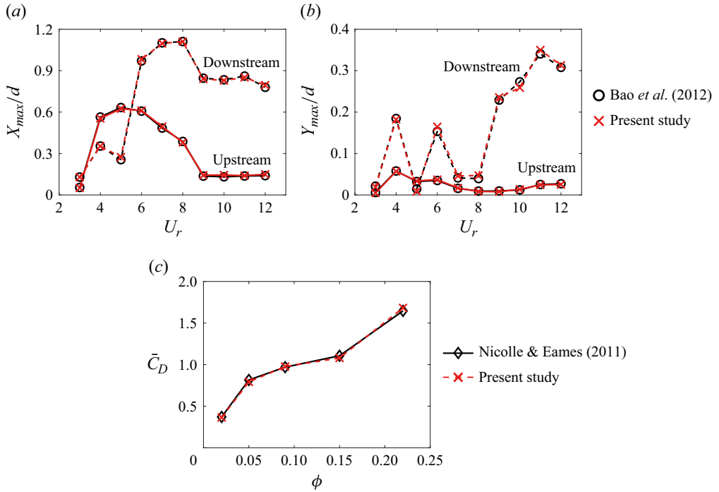
Figure 3. Comparison of maximum amplitudes (a) X_{max}/d and (b) Y_{max}/d with respect to reduced velocity U_r for two tandem cylinders ( \bar{m}^* = 2, Re_d = 150 ) undergoing vortex-induced vibration. (c) Comparison of time-averaged drag coefficient \bar{C}_D with respect to solid fraction \phi for a stationary cluster at Re_d = 100 .
